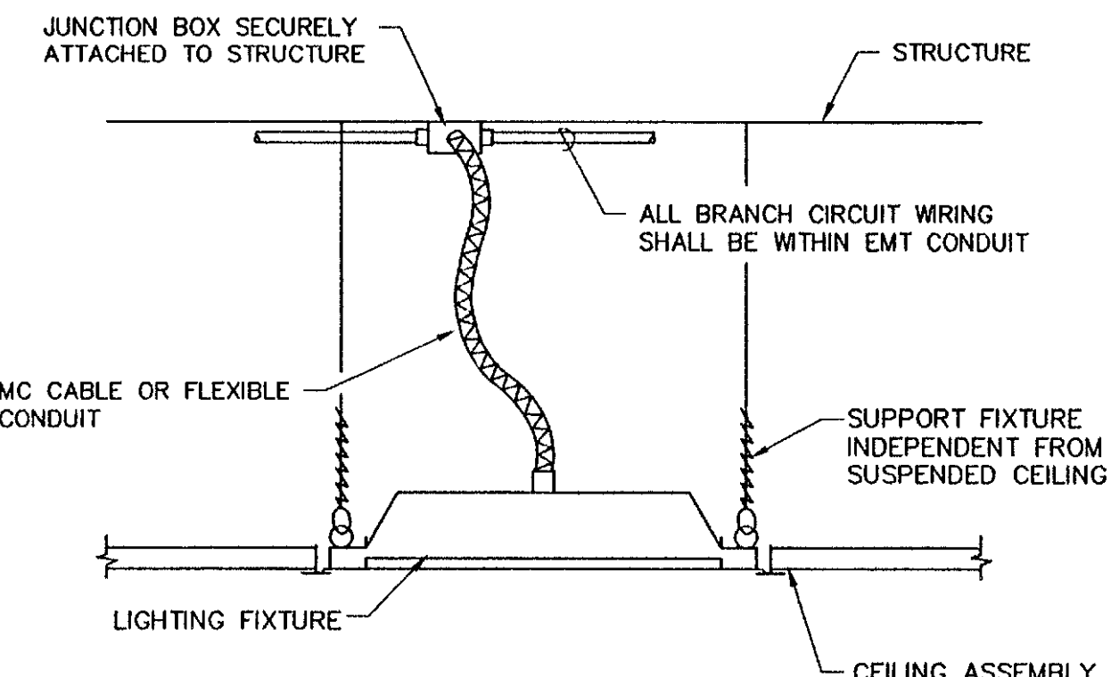
TYPICAL MOUNTING DETAIL FOR LIGHTING FIXTURE TYPES 'B', 'C' AND 'D' NOT TO SCALE
