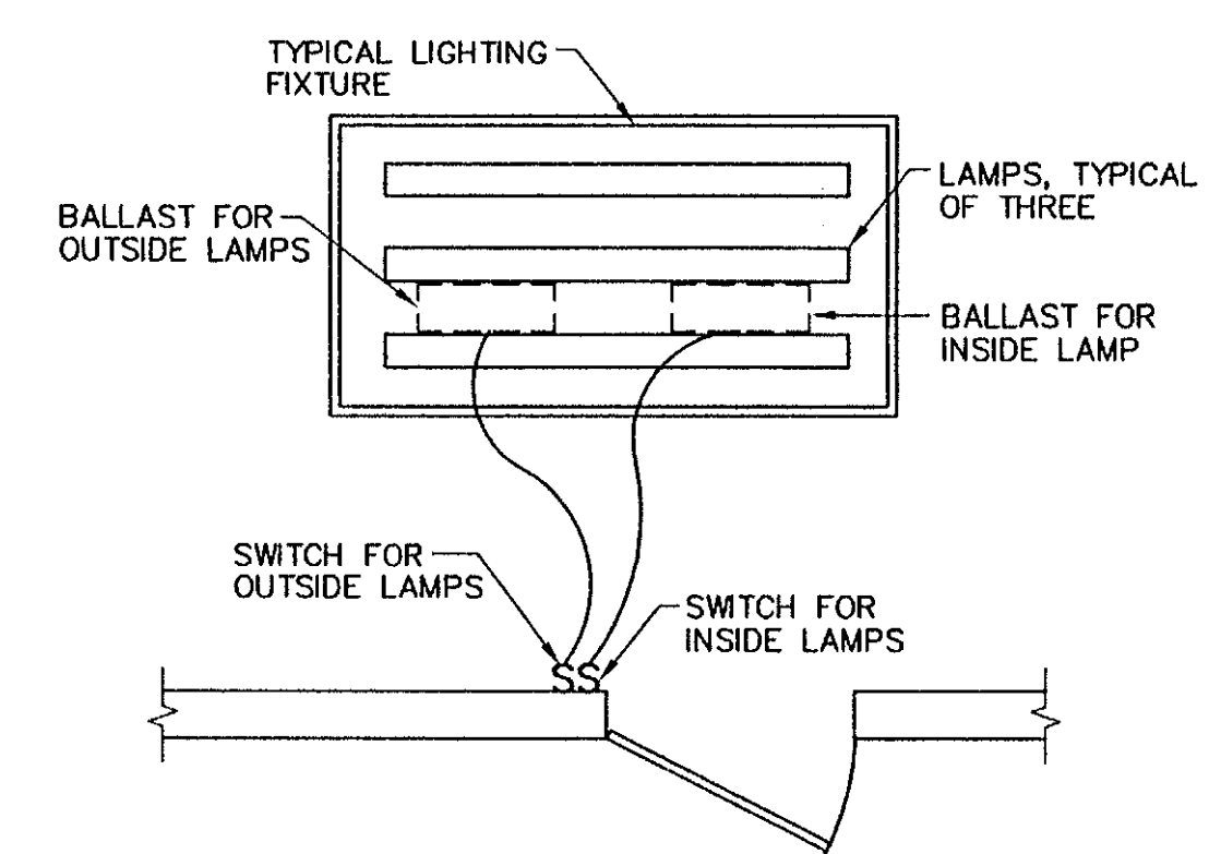
2-SWITCH CONTROL OF LIGHT FIXTURES NOT TO SCALE
