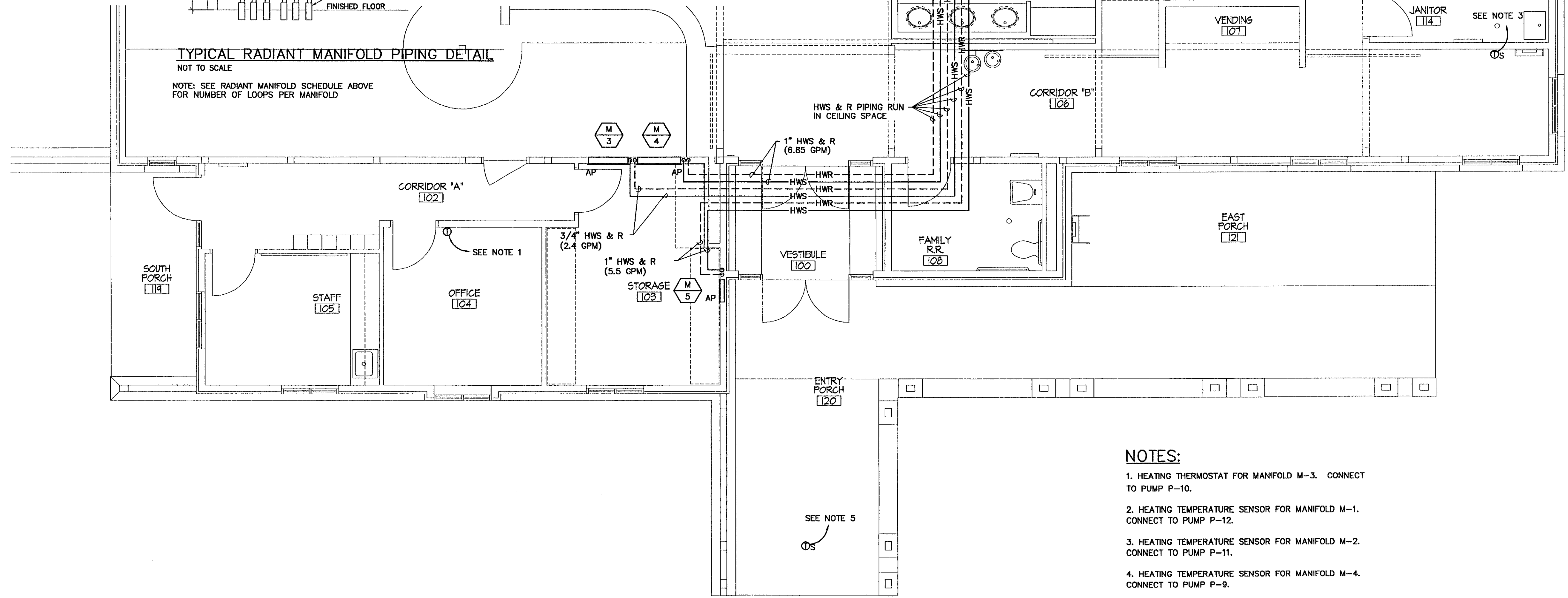
PIPING PLAN SCALE: 1/4"=1'-0"
