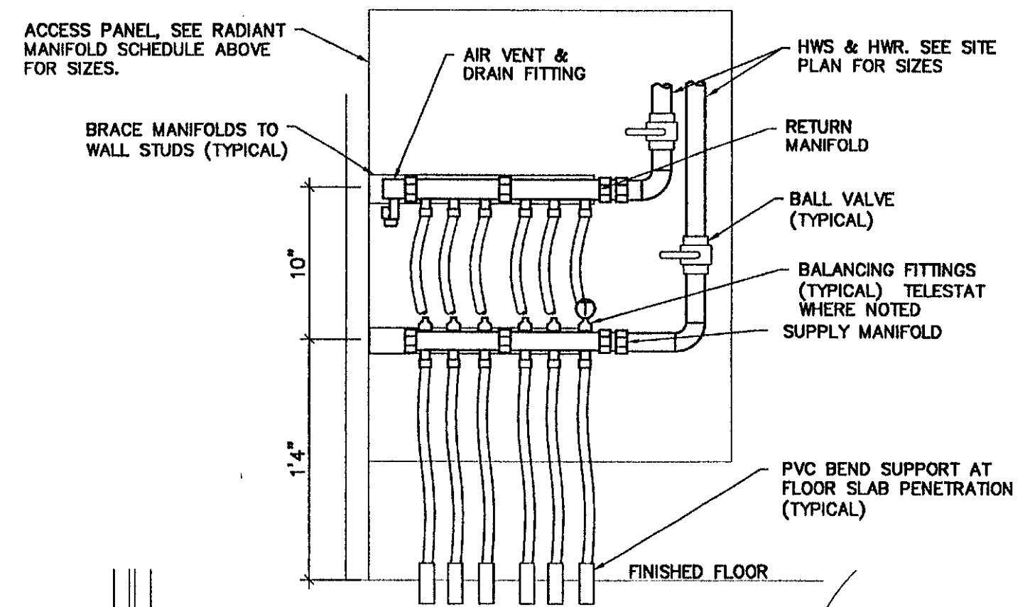
TYPICAL RADIANT MANIFOLD PIPING DETAIL NOT TO SCALE NOTE: SEE RADIANT MANIFOLD SCHEDULE ABOVE FOR NUMBER OF LOOPS PER MANIFOLD
