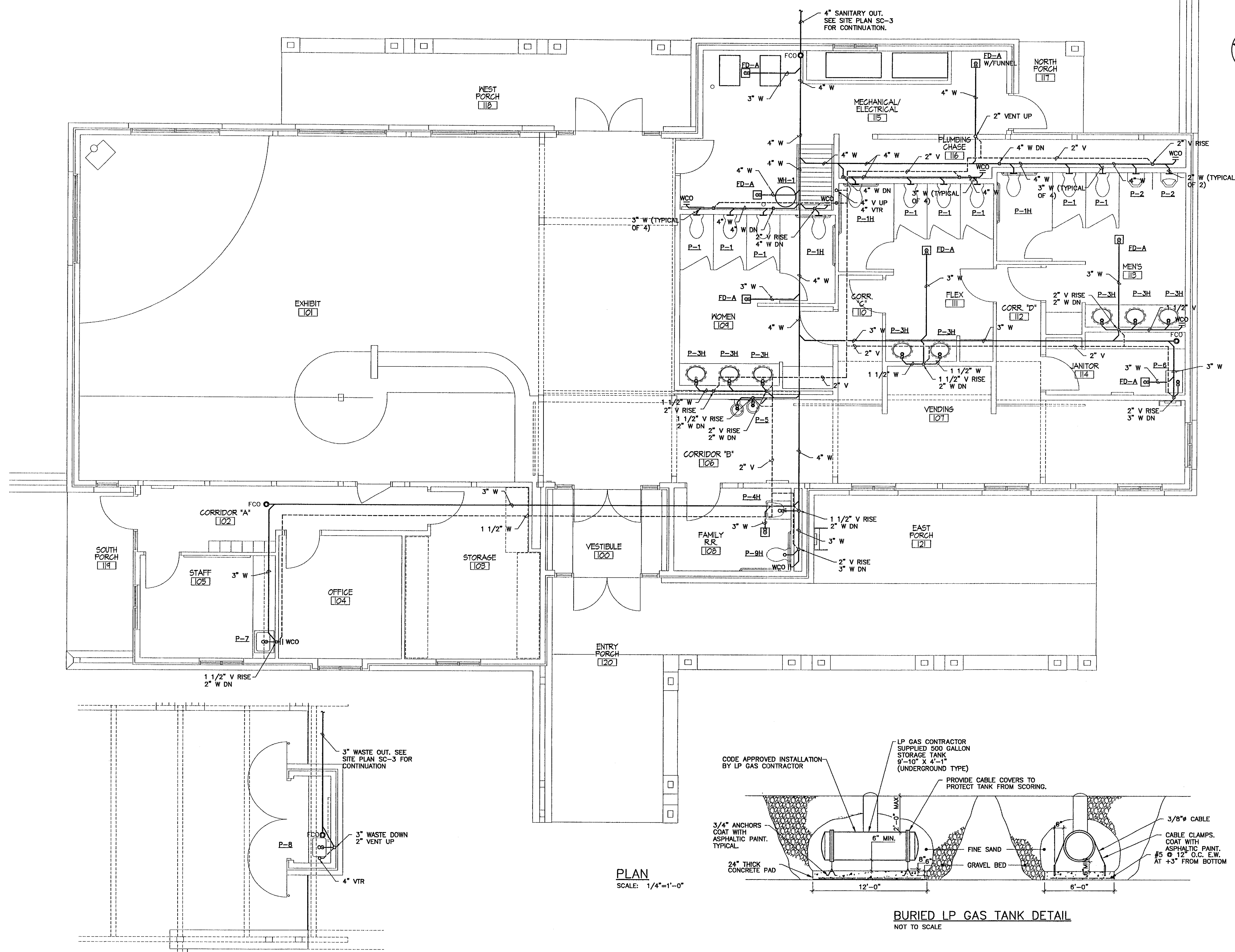
WASTE AND VENT PIPING PLAN - PAVILION SCALE: 1/4"=1'-0"
