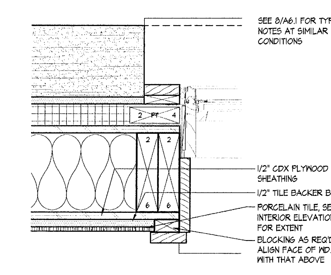
4 WINDOW JAMB AT TILE SCALE: 3" = 1'-0" 2003_DTL-TILE01
