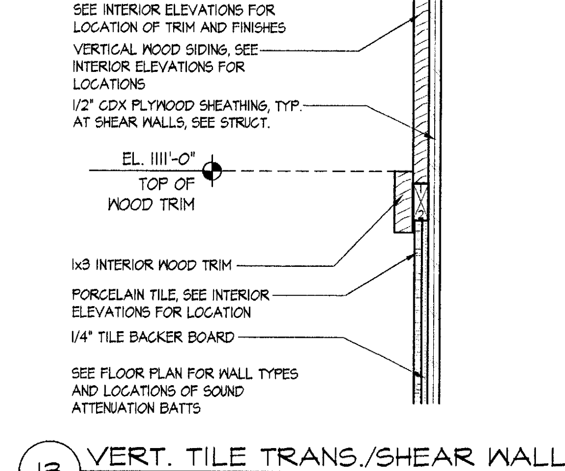
13 TILE TO TILE BASE DETAIL SCALE: 3" = 1'-0" 2003_DTL-TILE01
