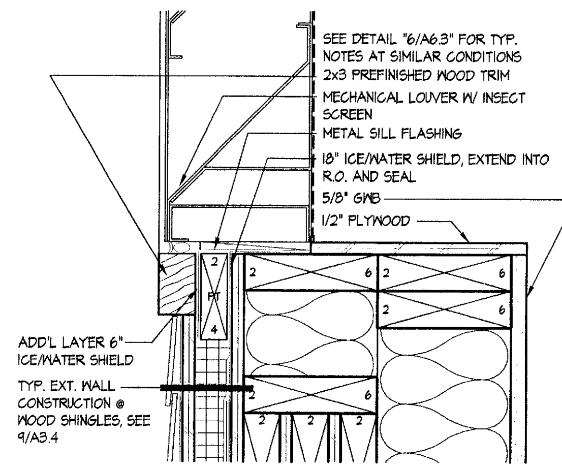
7 CIRCLE LOUVER SILL DETAIL SCALE: 3" = 1'-0" 2003_DTL-LOUVER
