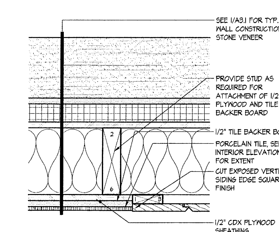
9 HORIZONTAL TILE TRANSITION SCALE: 3" = 1'-0" 2003_DTL-TILE01
