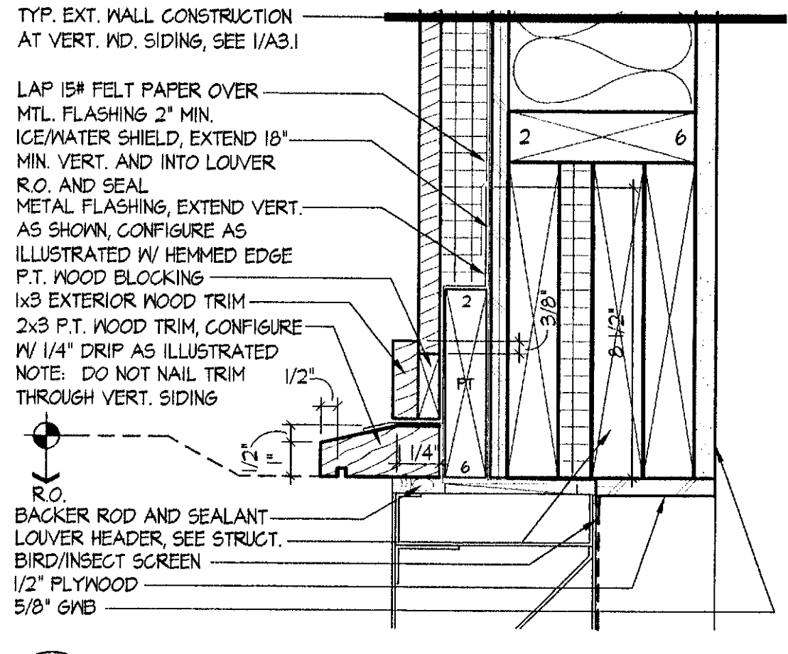
1 LOUVER HEAD DETAIL SCALE: 3" = 1'-0" 2003_DTL-LOUVER
