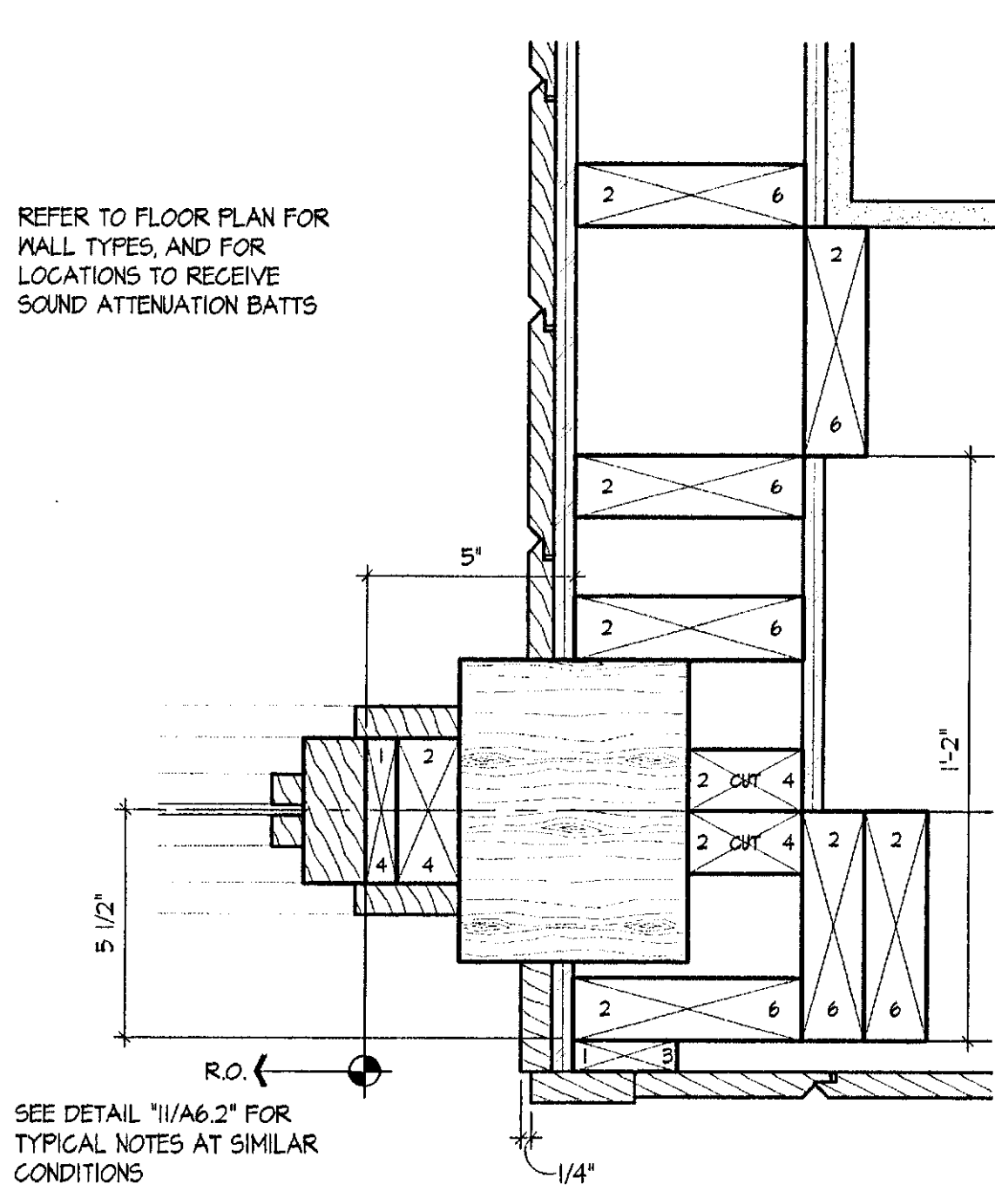
10 INTERIOR WINDOW JAMB SCALE: 3" = 1'-0" 2003_DTL-WINDW02
