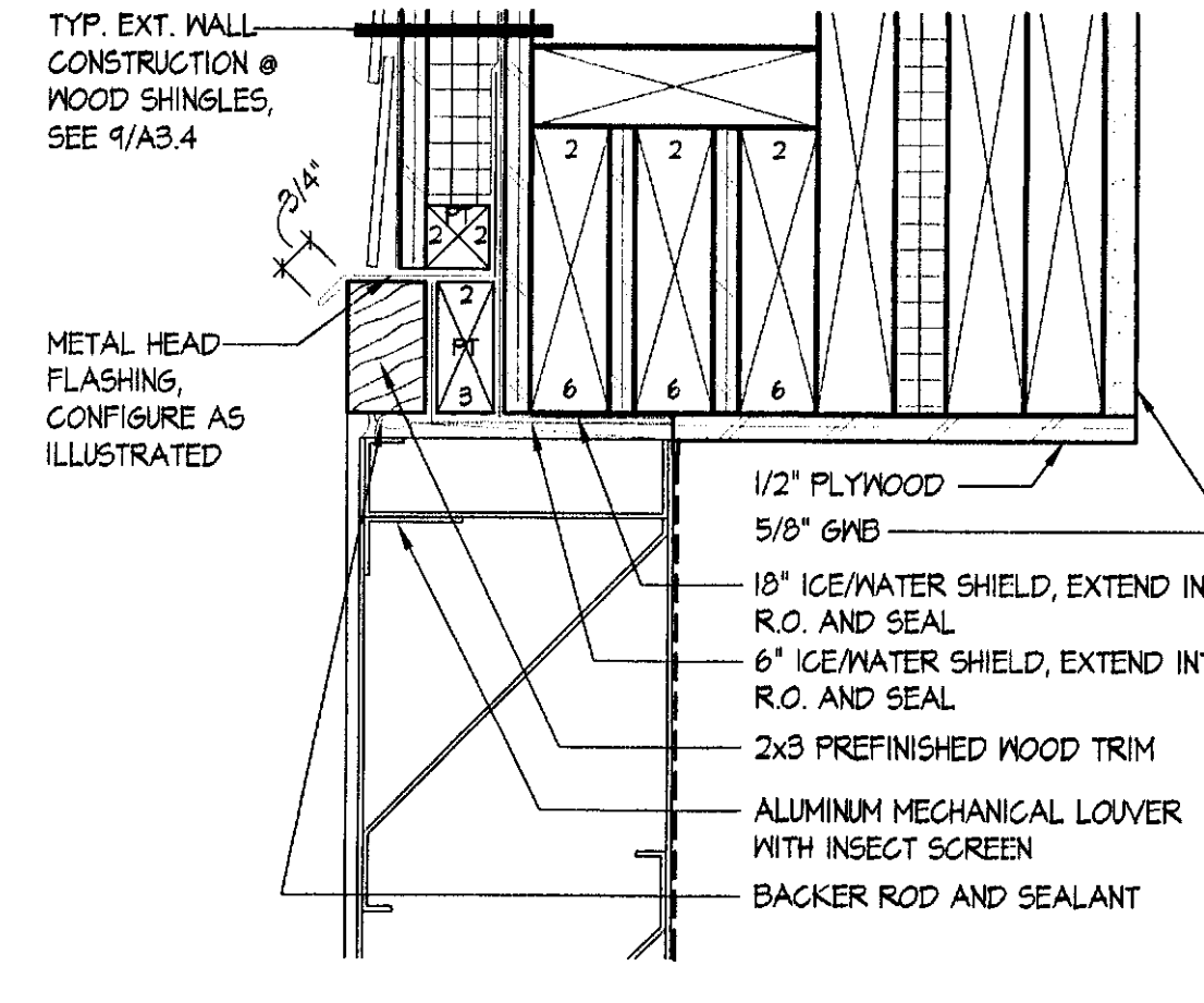
2 CIRCLE LOUVER HEAD DETAIL SCALE: 3" = 1'-0" 2003_DTL-LOUVER
