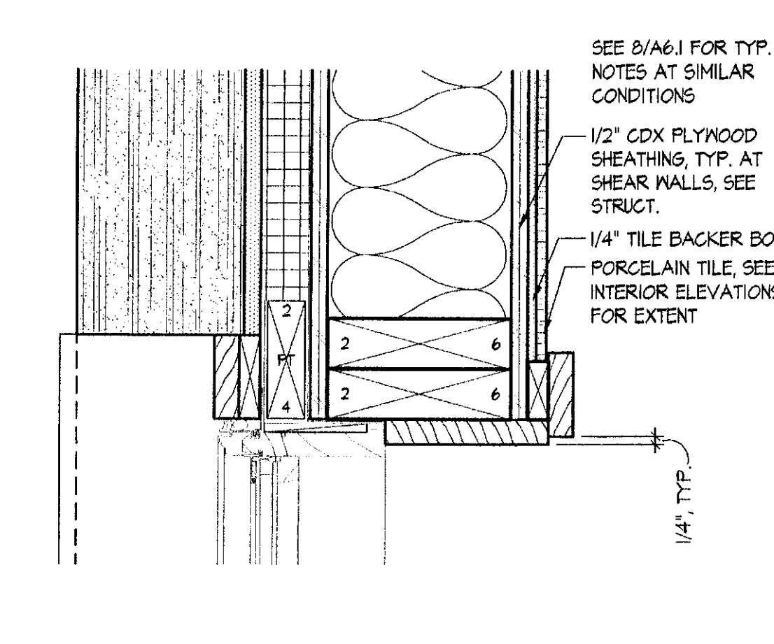
3 WINDOW JAMB/SHEAR WALL @ TILE SCALE: 3" = 1'-0" 2003_DTL-TILE01
