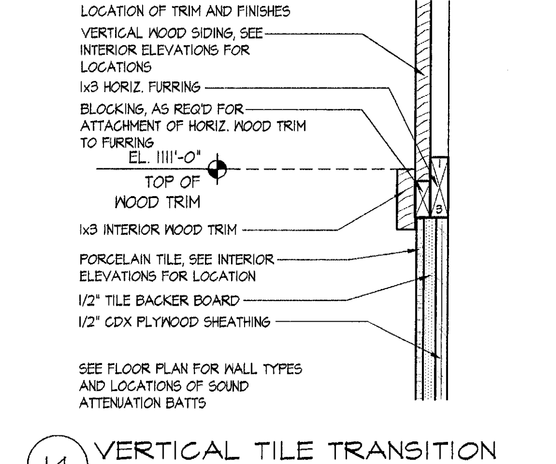
14 TILE TO TILE BASE DETAIL SCALE: 3" = 1'-0" 2003_DTL-TILE01
