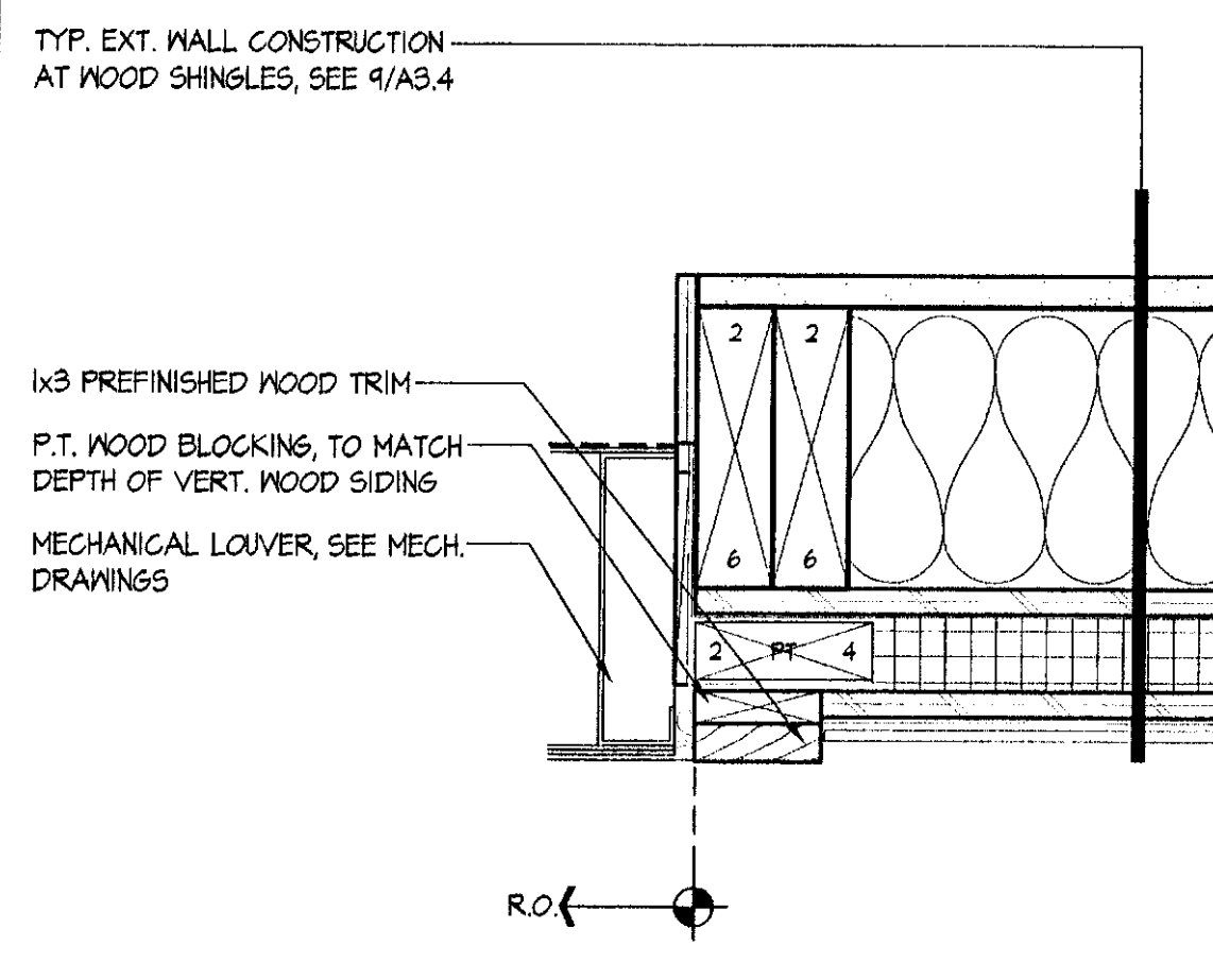
5 LOUVER JAMB DETAIL SCALE: 3" = 1'-0" 2003_DTL-LOUVER
