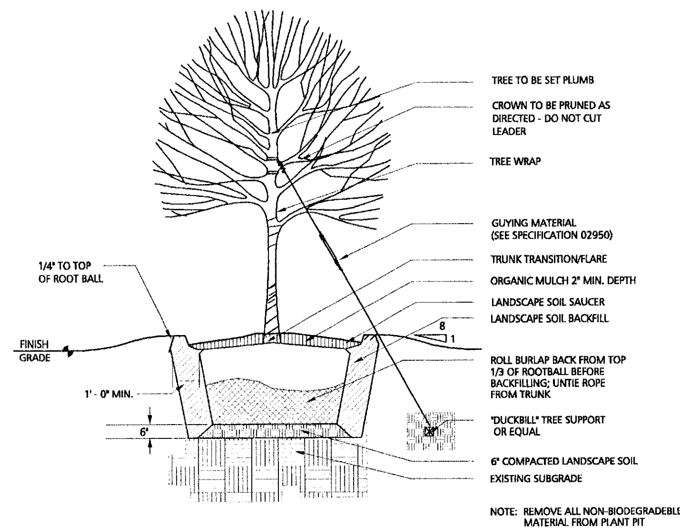
1 L2 DECIDUOUS TREE PLANTING DETAIL NTS
