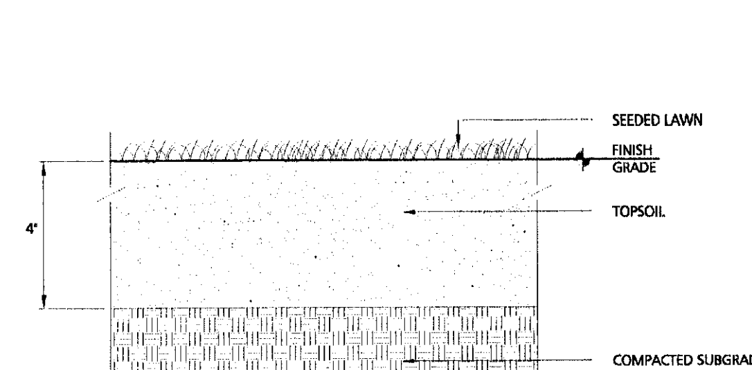
4 L2 SEED LAWN DETAIL NTS
