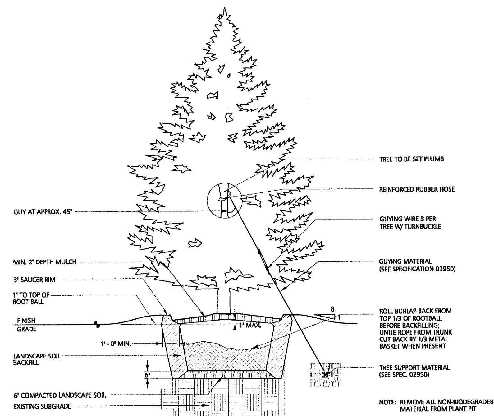
2 L2 EVERGREEN TREE PLANTING DETAIL NTS
