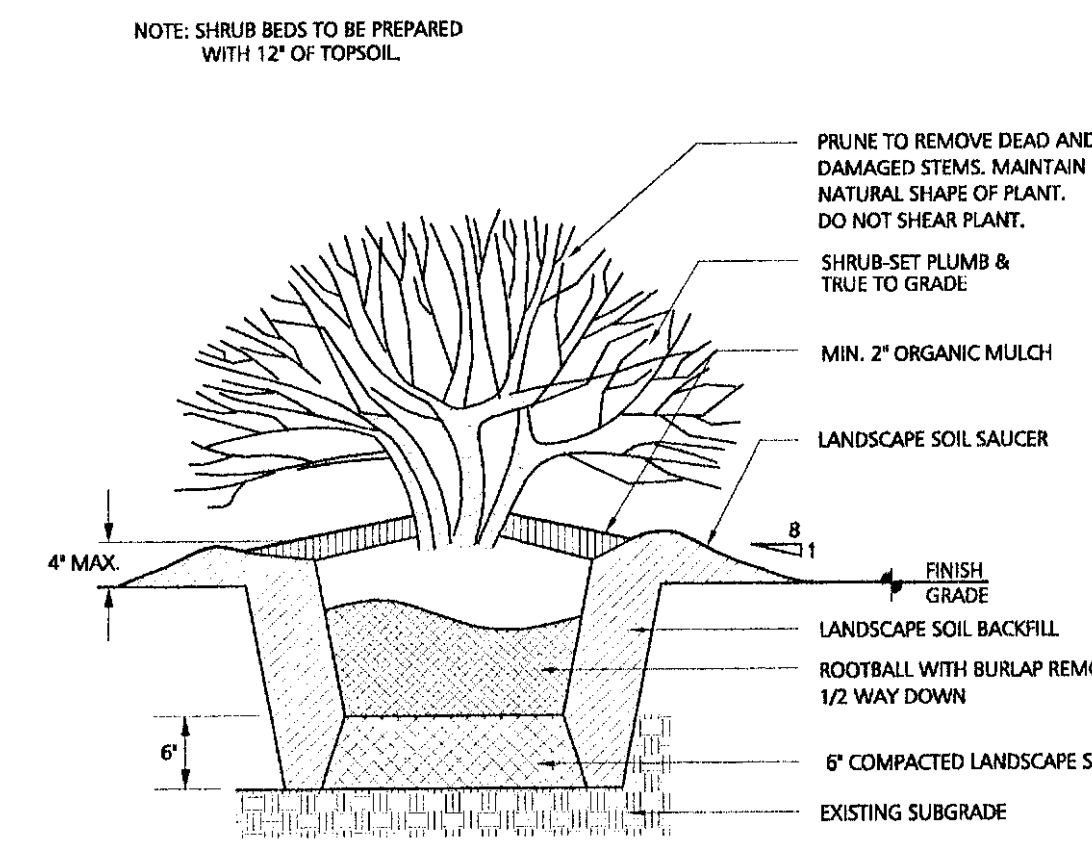
3 L2 SHRUB PLANTING DETAIL NTS
