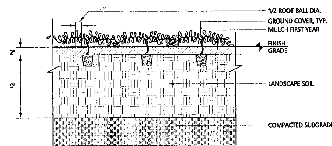
5 L2 GROUND COVER PLANTING DETAIL NTS
