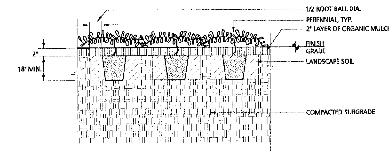
6 L2 PERENNIAL PLANTING DETAIL NTS
