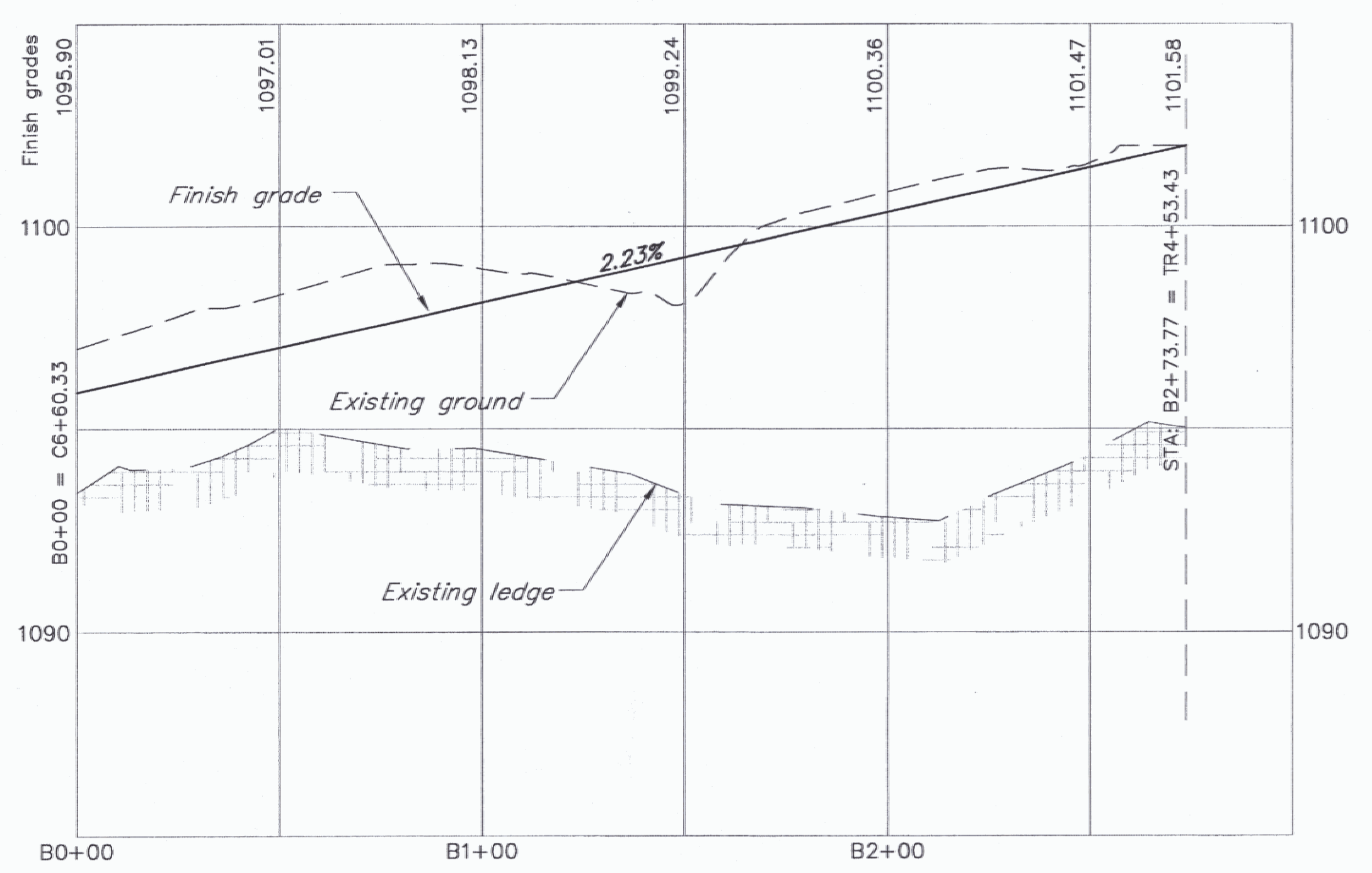
"B" Lane Profile Scales: Horiz. 1" = 30' Vert. 1" = 3'
