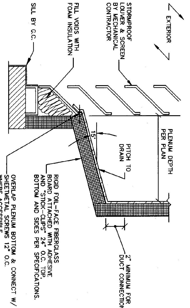
PLENUM AT LOUVER DETAIL SCALE: NONE
