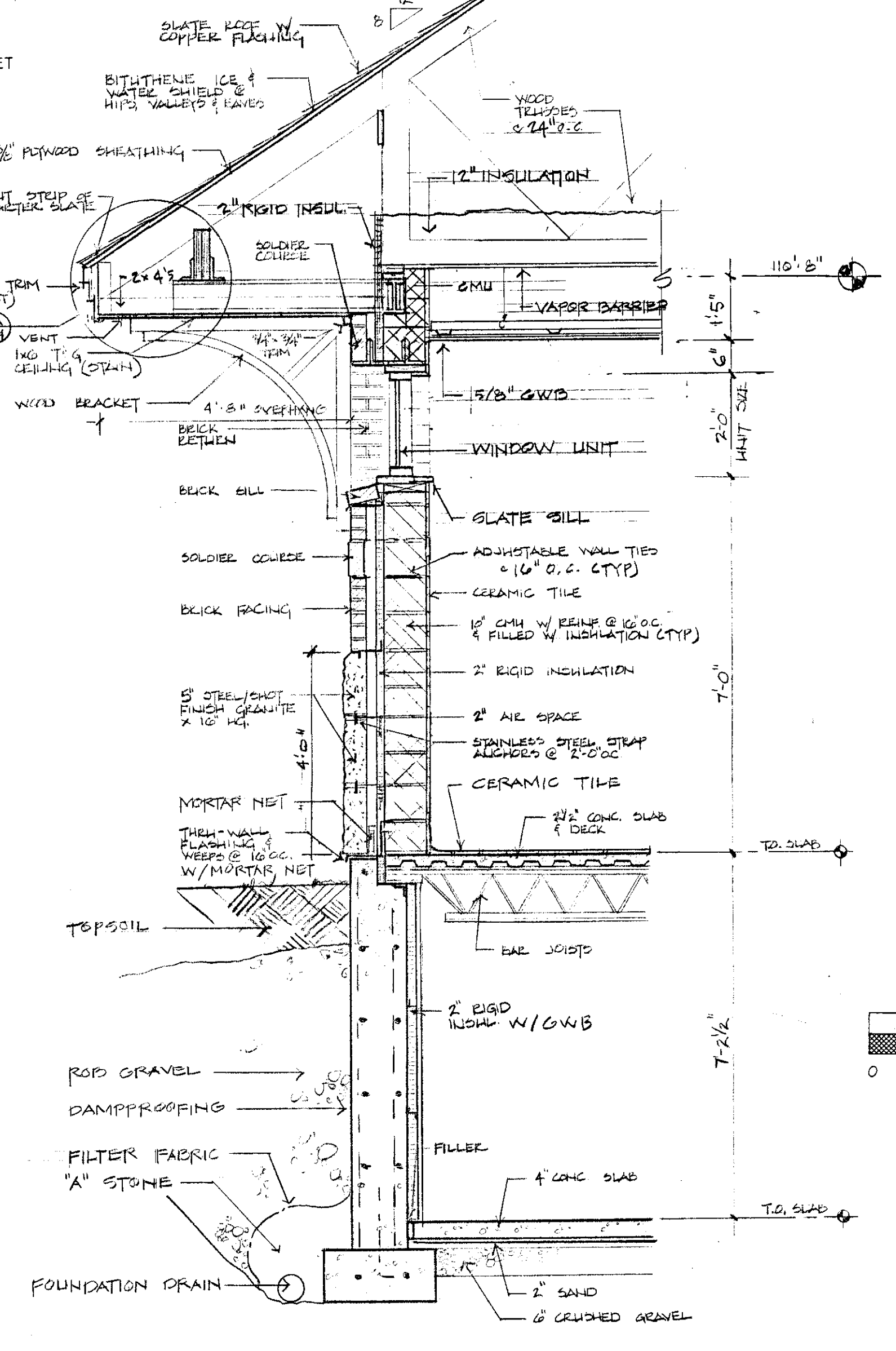
2 WALL SECTION @ TOILET RM. 1/2" = 1'-0"
