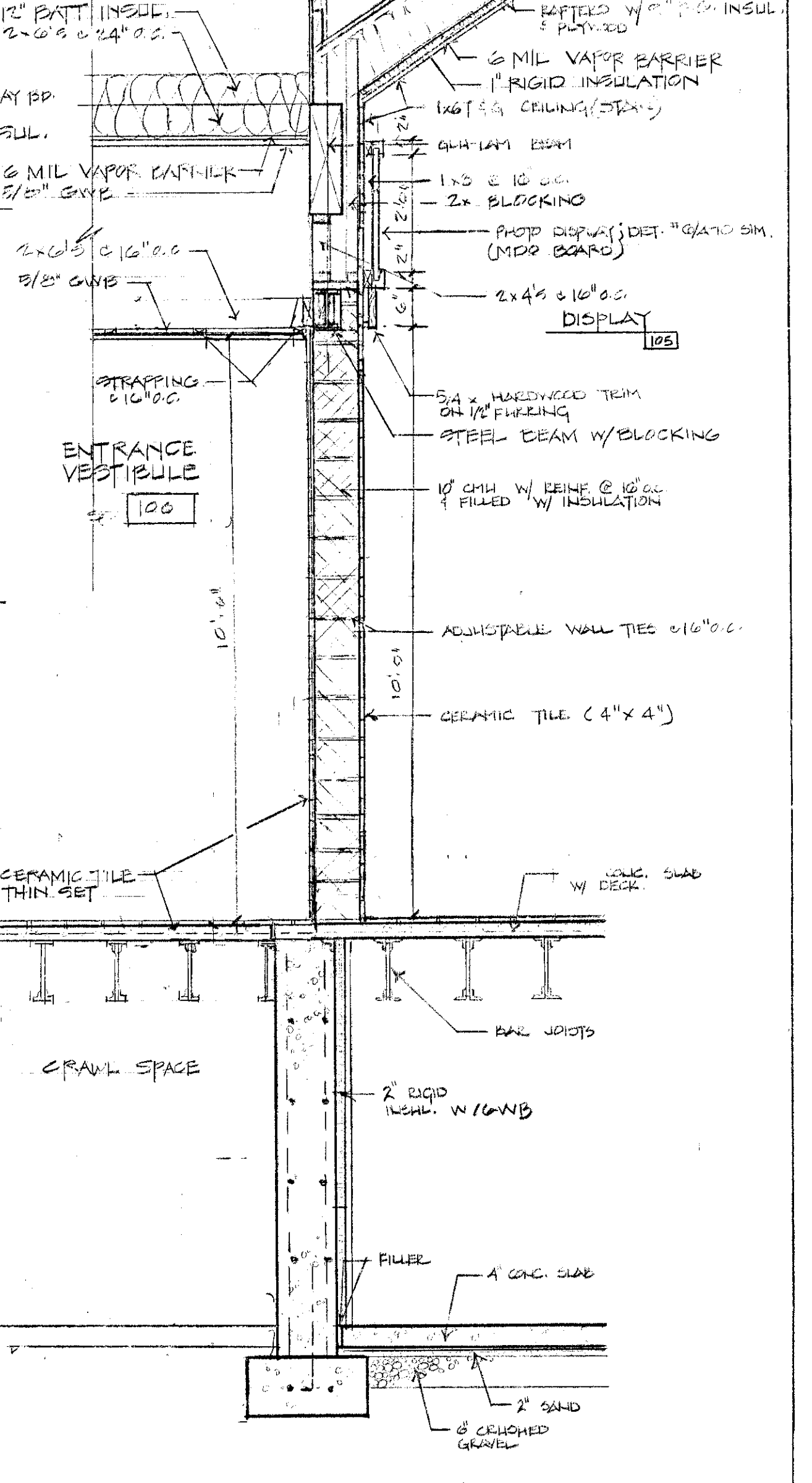
4 WALL SECTION @ FRONT 1/2" = 1'-0"
