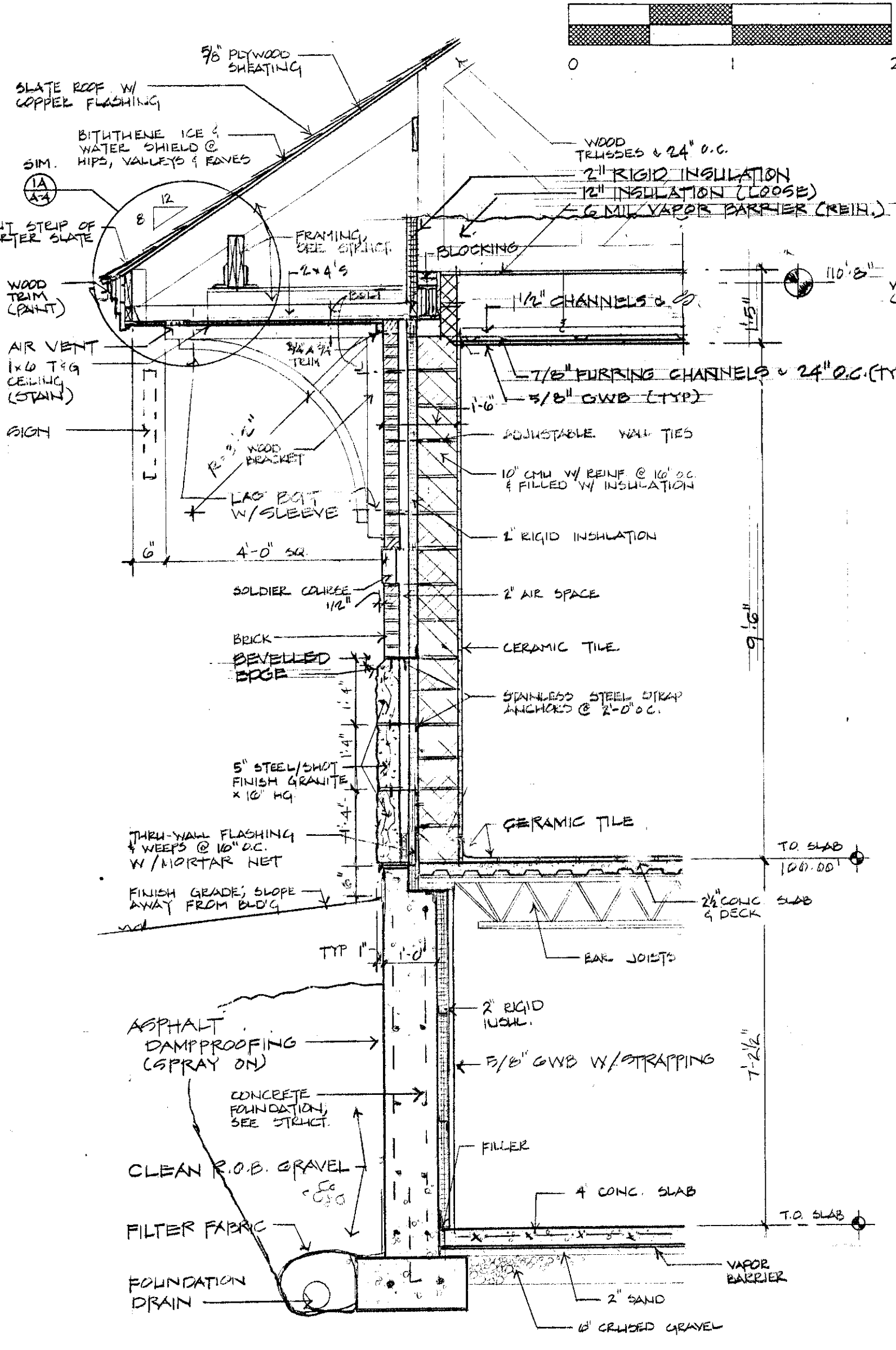
1 TYPICAL WALL SECTION 1/2" = 1'-0"
