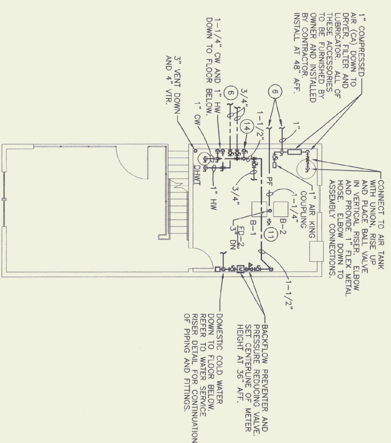
SECOND FLOOR PLAN SCALE: 1/8" = 1'-0"
