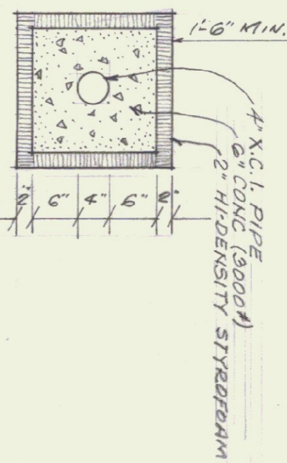
SECTION THRU SOIL PIPE UNDER DRIVEWAY SCALE: 3/4" = 1'-0"
