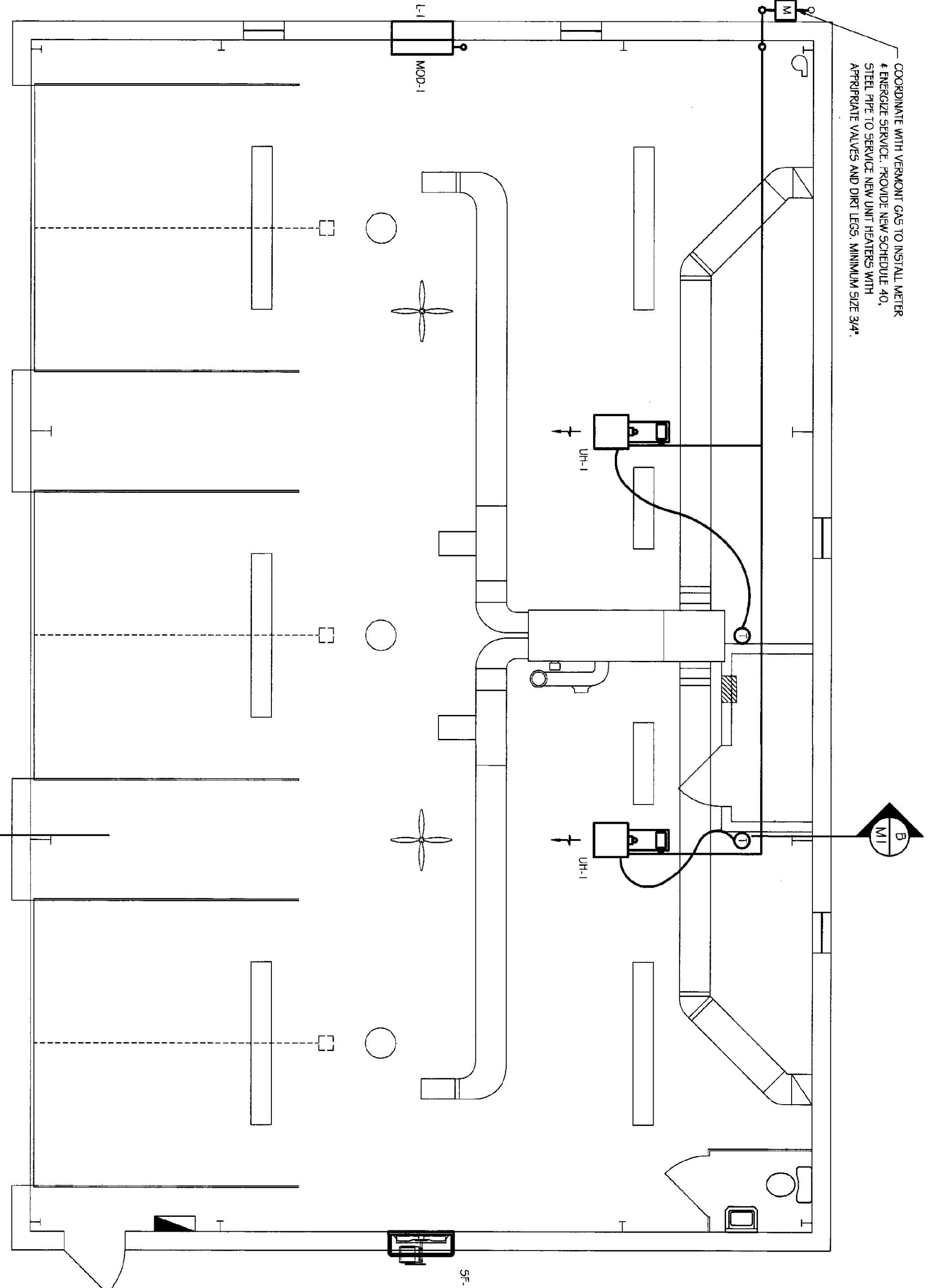
NEW HEATING PLAN SCALE: 1/4"=1'-0"
