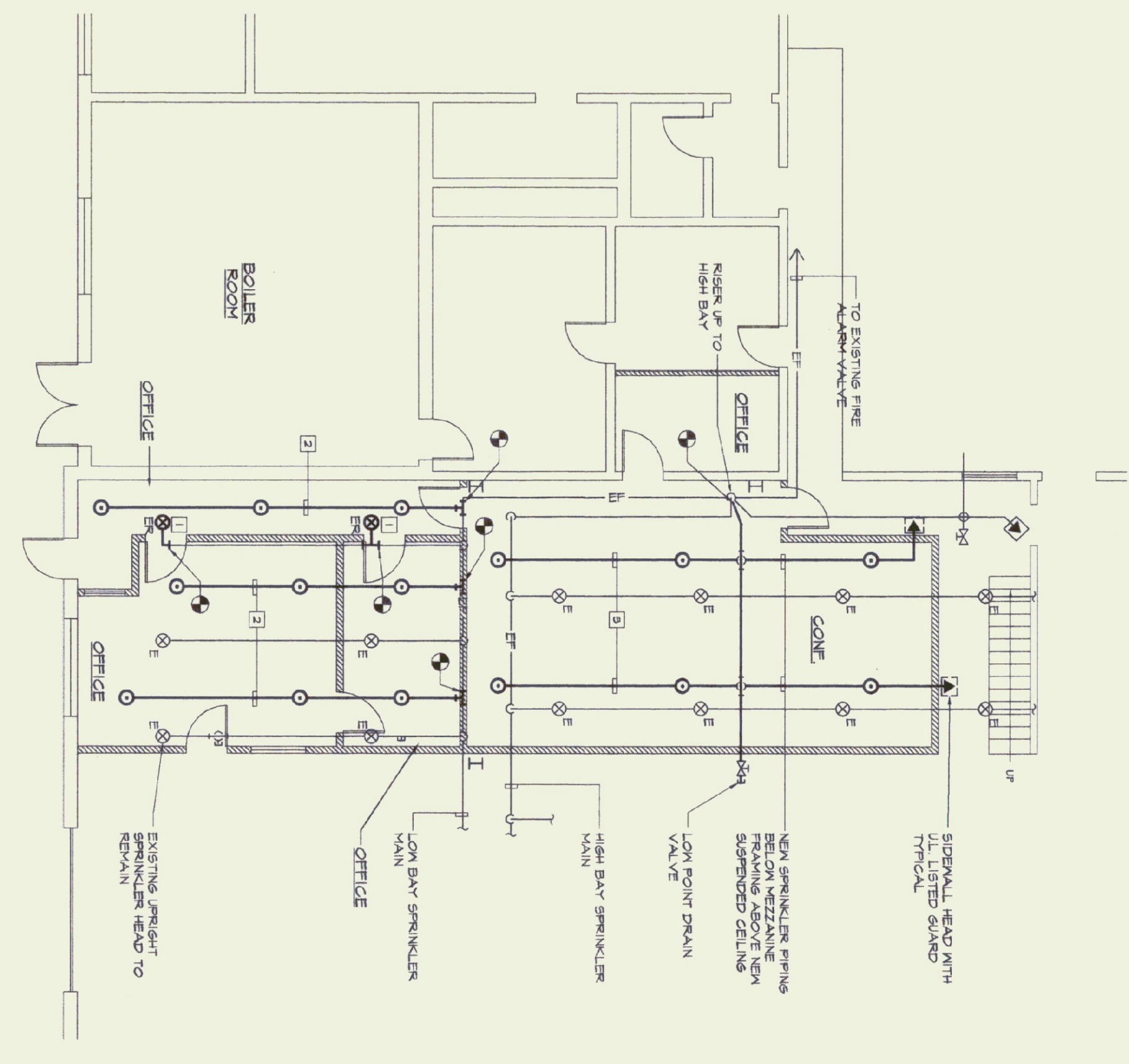
PARTIAL MAIN FLOOR PLAN - FIRE PROTECTION NEW WORK SCALE: 1/8"=1'-0"
