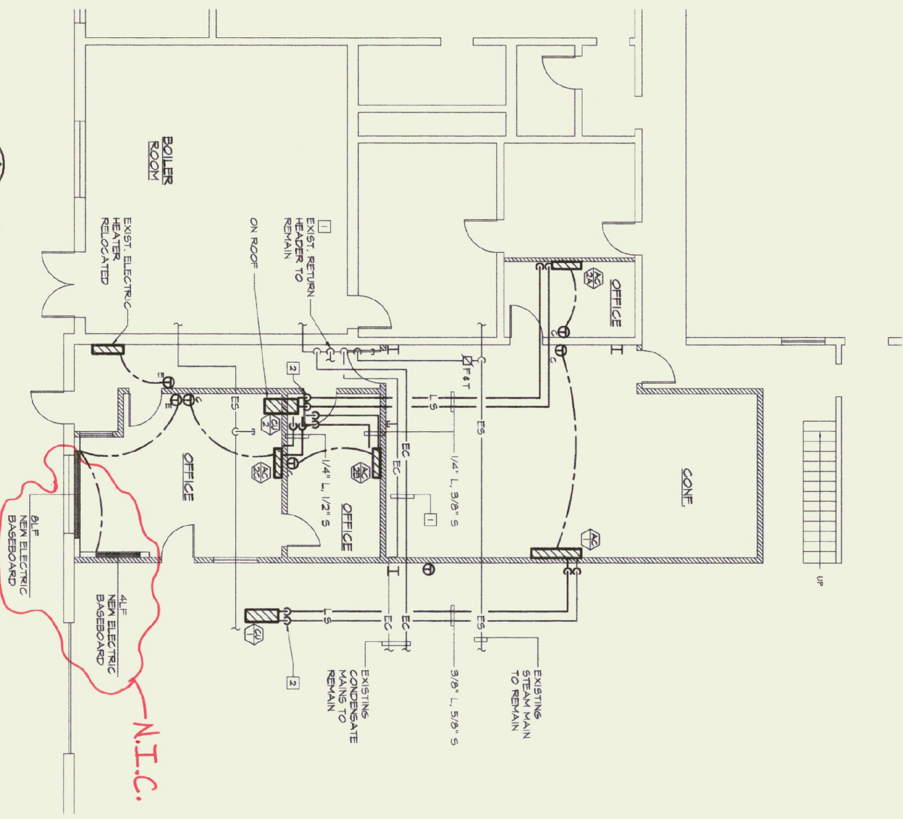
PARTIAL MAIN FLOOR PLAN - HVAC NEW WORK SCALE: 1/8"=1'-0"
