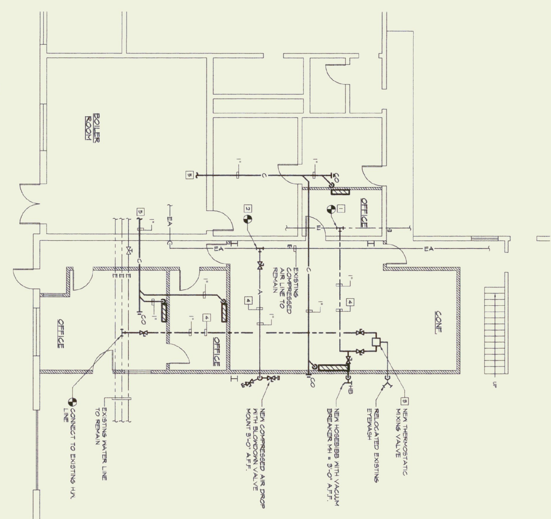
PARTIAL MAIN FLOOR PLAN - PLUMBING NEW WORK SCALE: 1/8"=1'-0"
