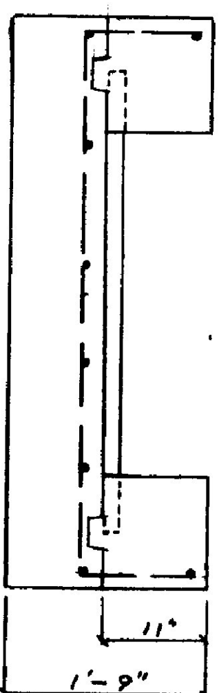
ALTERNATE BRANCH TRENCH DESIGN
