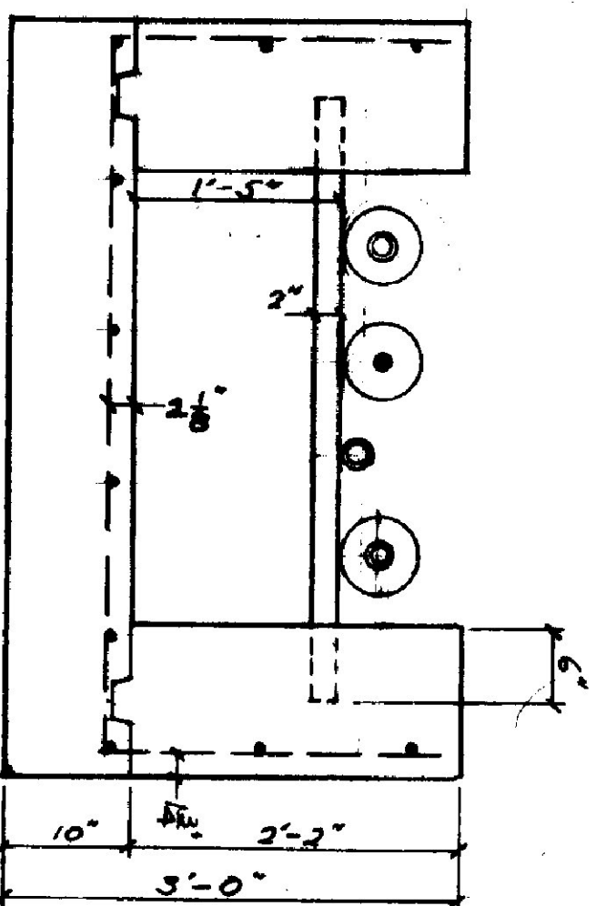
SECTION AT SUPPORT (BRANCH)
