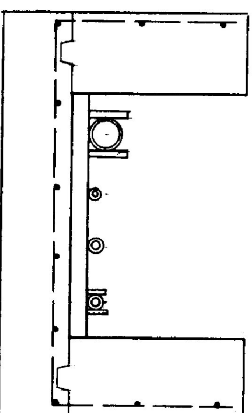
SECTION AT ALTERNATE GUIDE (MAIN)
