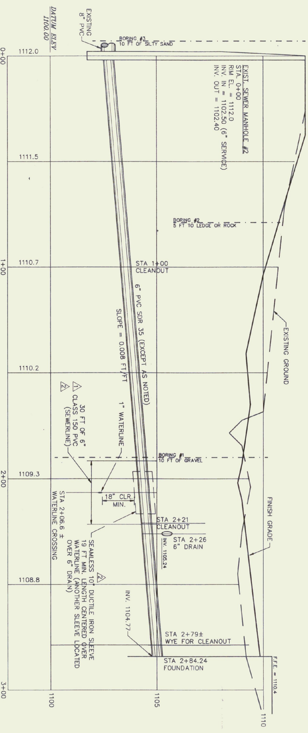
PROFILE 12 SCALE: 1\"/>
