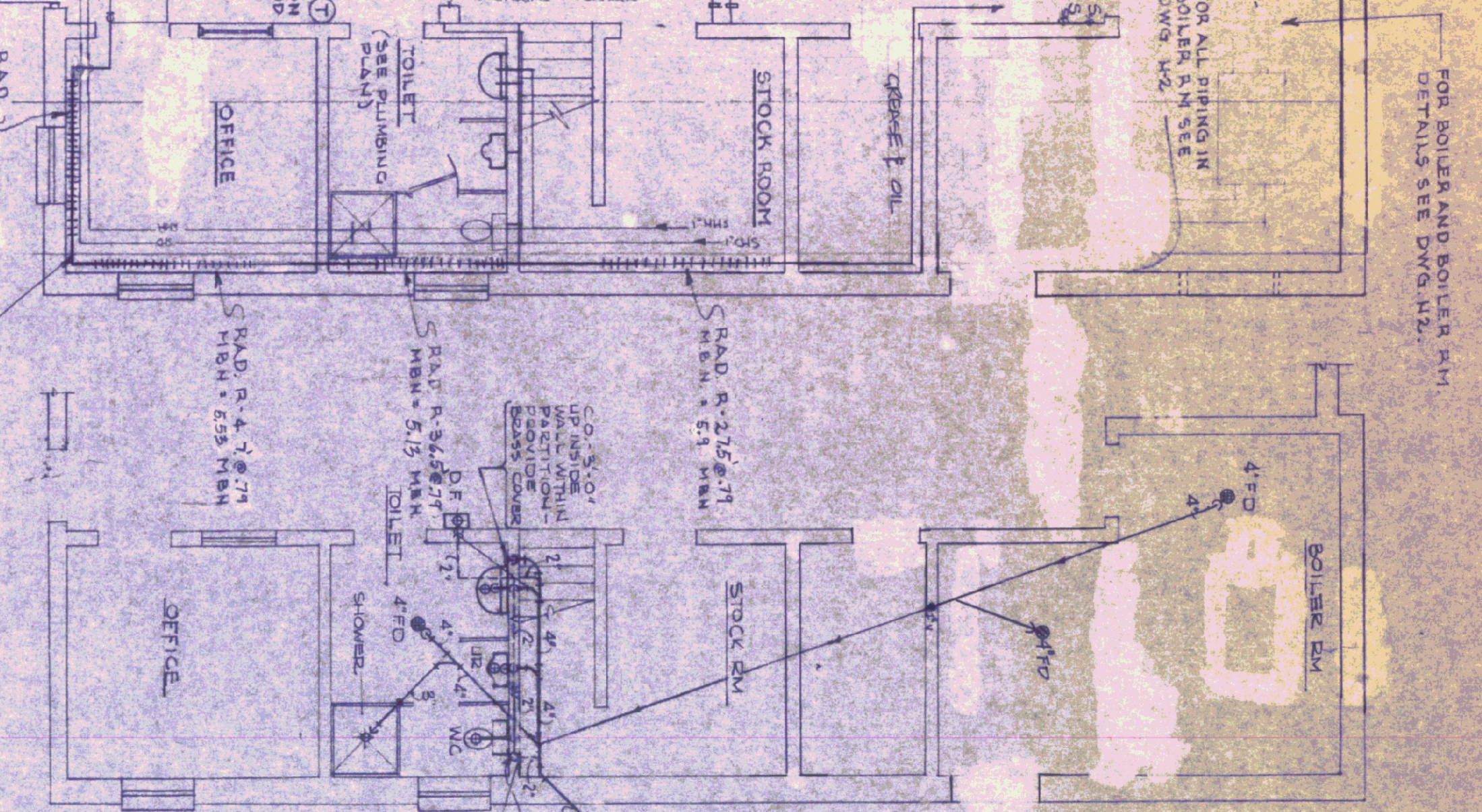
PLUMBING PLAN SCALE: 1/16"
