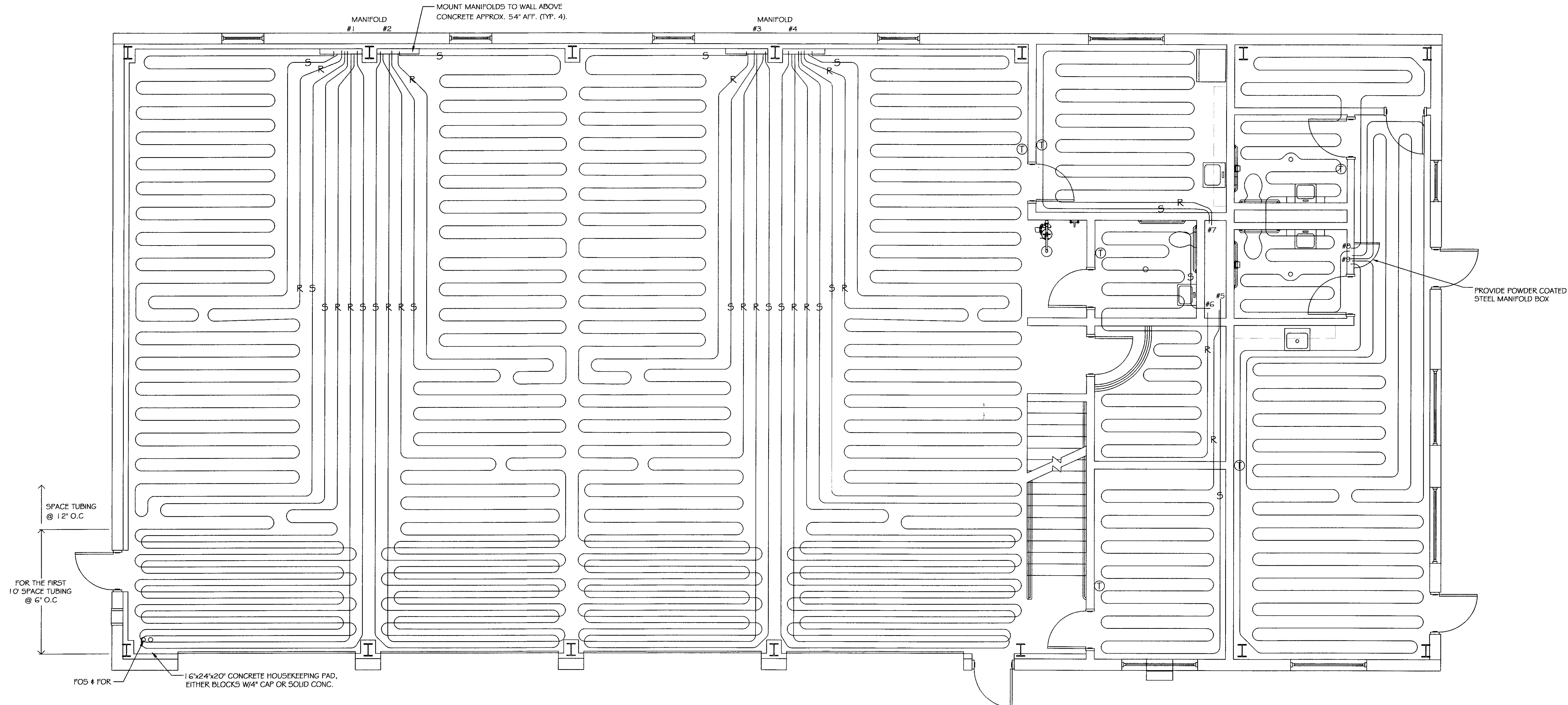
FIRST FLOOR RADIANT HEATING PLAN
