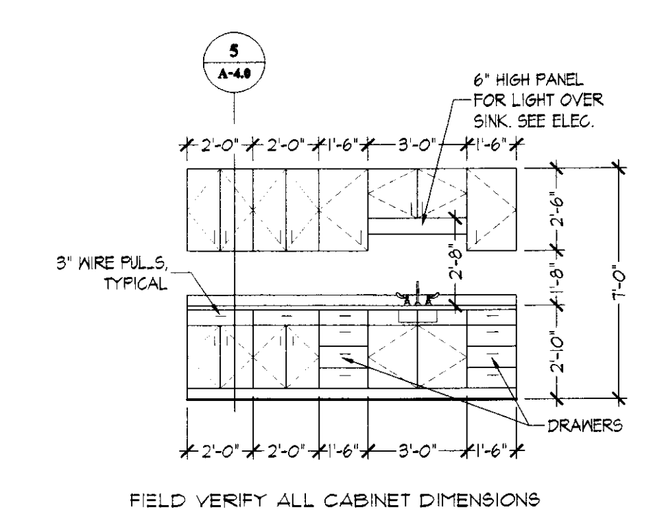
4 CABINET ELEV. @ BREAK ROOM 105 SCALE: 1/4" = 1'-0"
