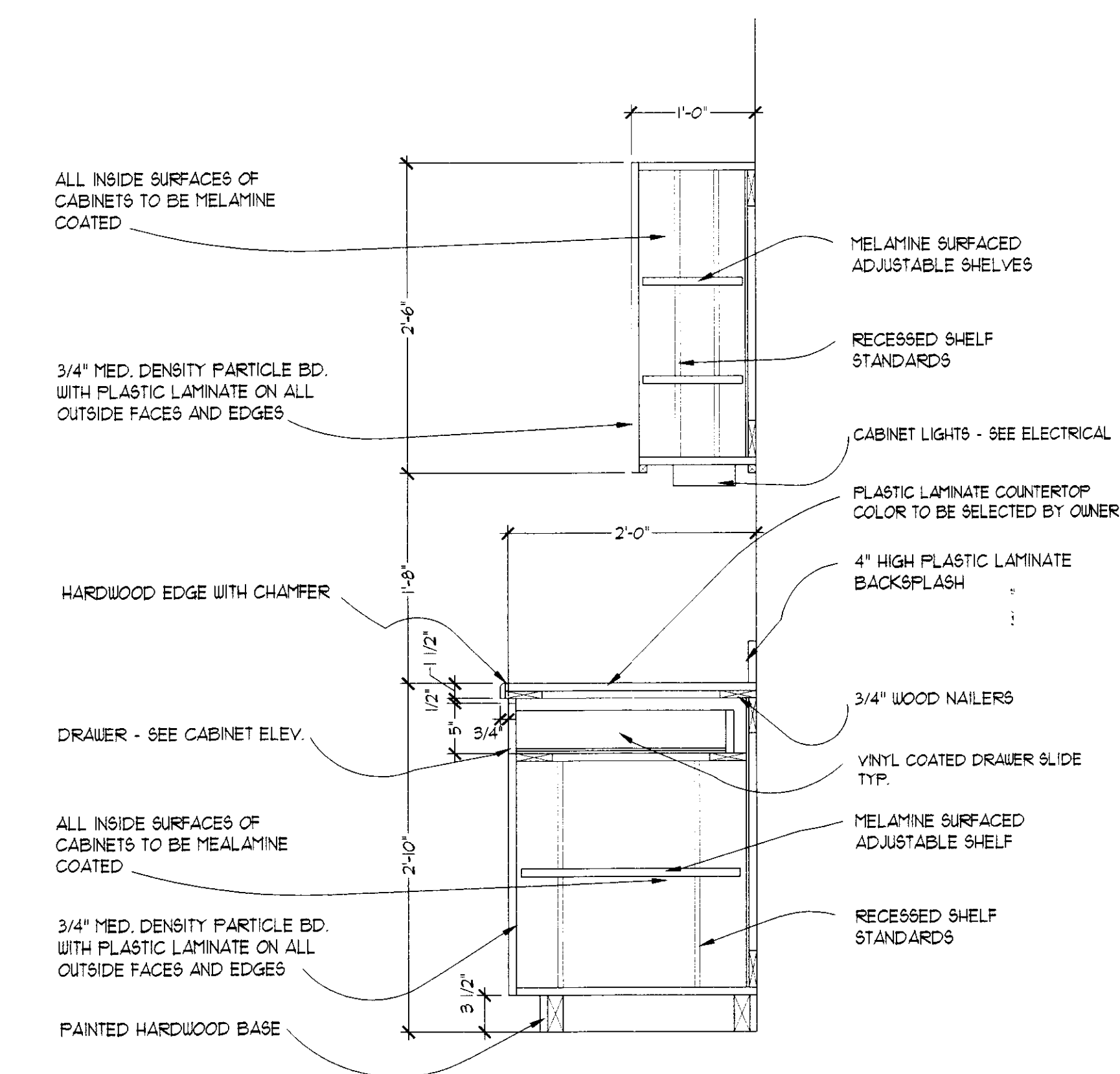
5 TYPICAL CABINET SECTION SCALE: 1" = 1'-0"
