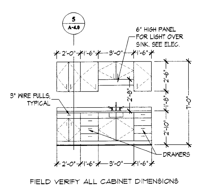
3 CABINET ELEV. @ ROOM 111 SCALE: 1/4" = 1'-0"
