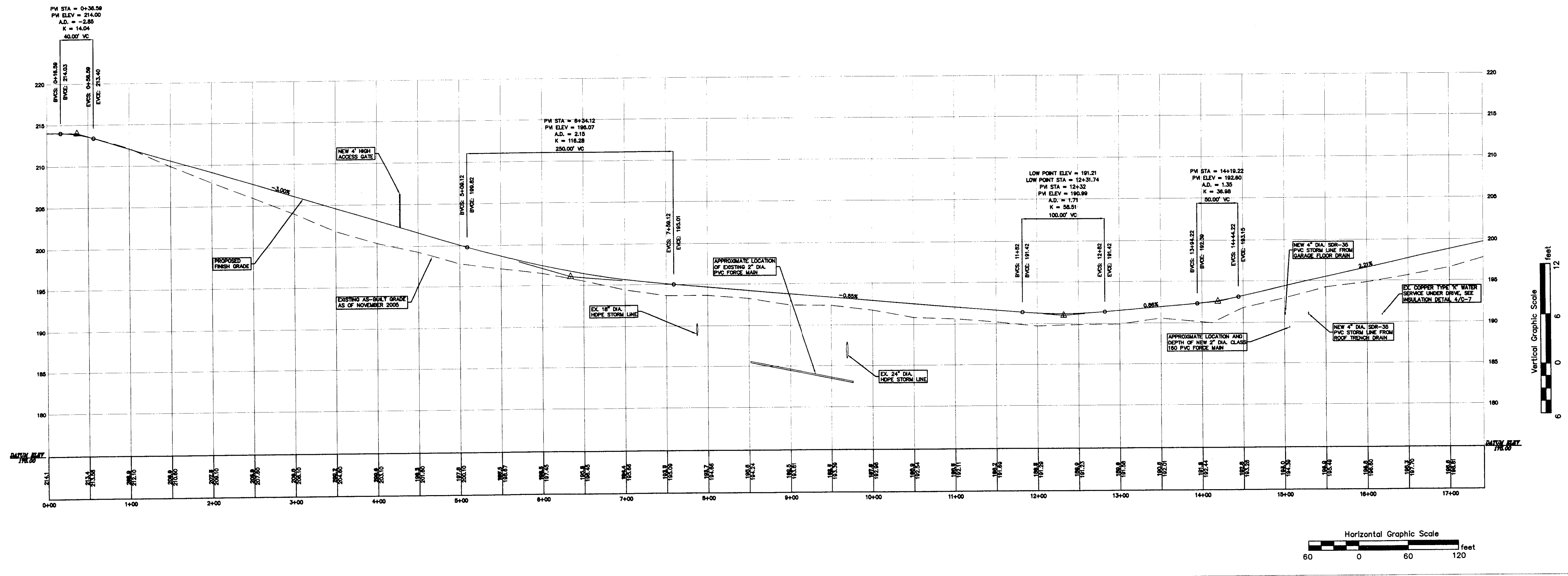
C-4 CENTERLINE DRIVEWAY PROFILE STA 0+00 TO 17+41
