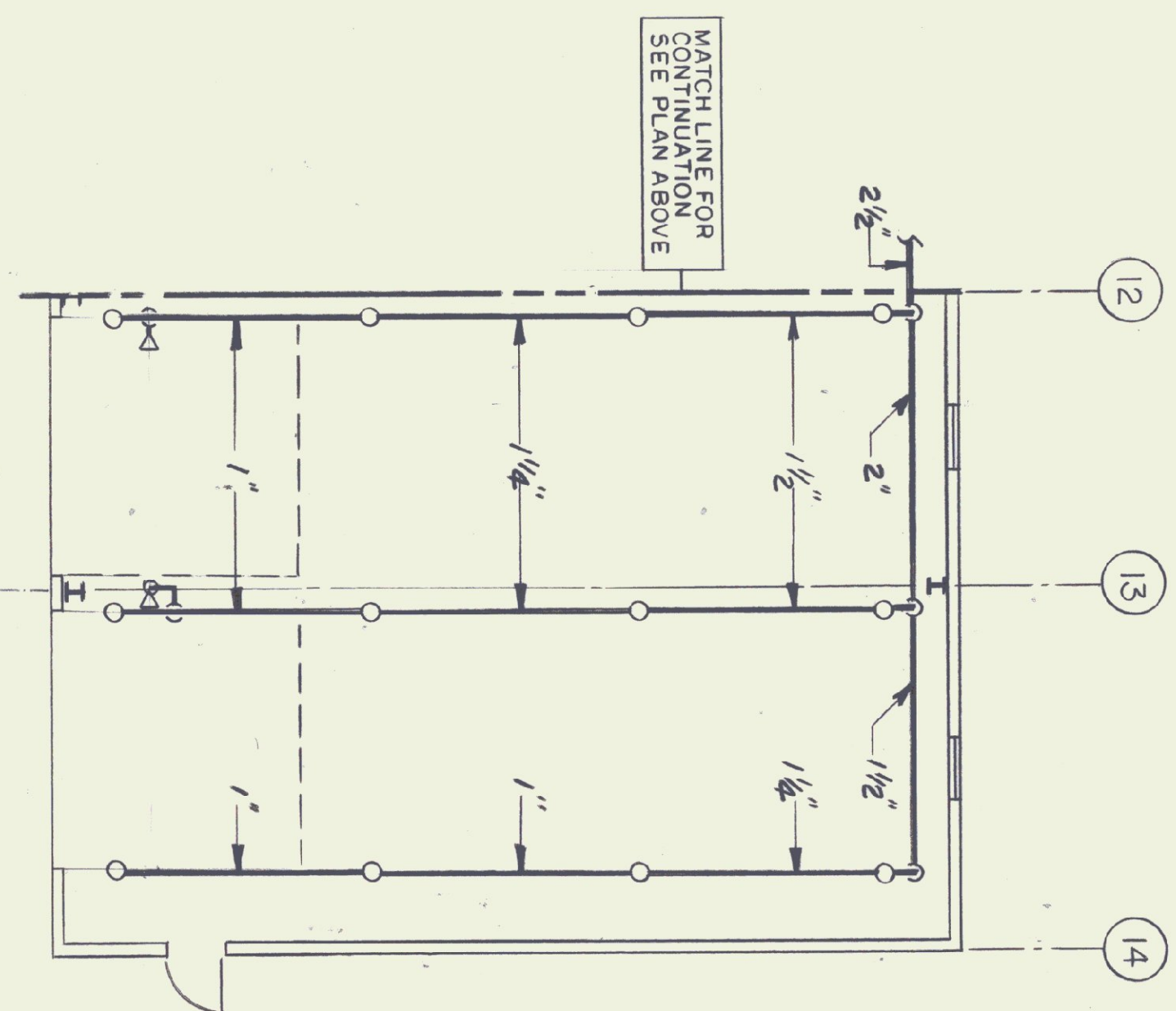
FIRE PROTECTION-PARTIAL MAIN LEVEL PLAN SCALE: 1/8"=1'-0"
