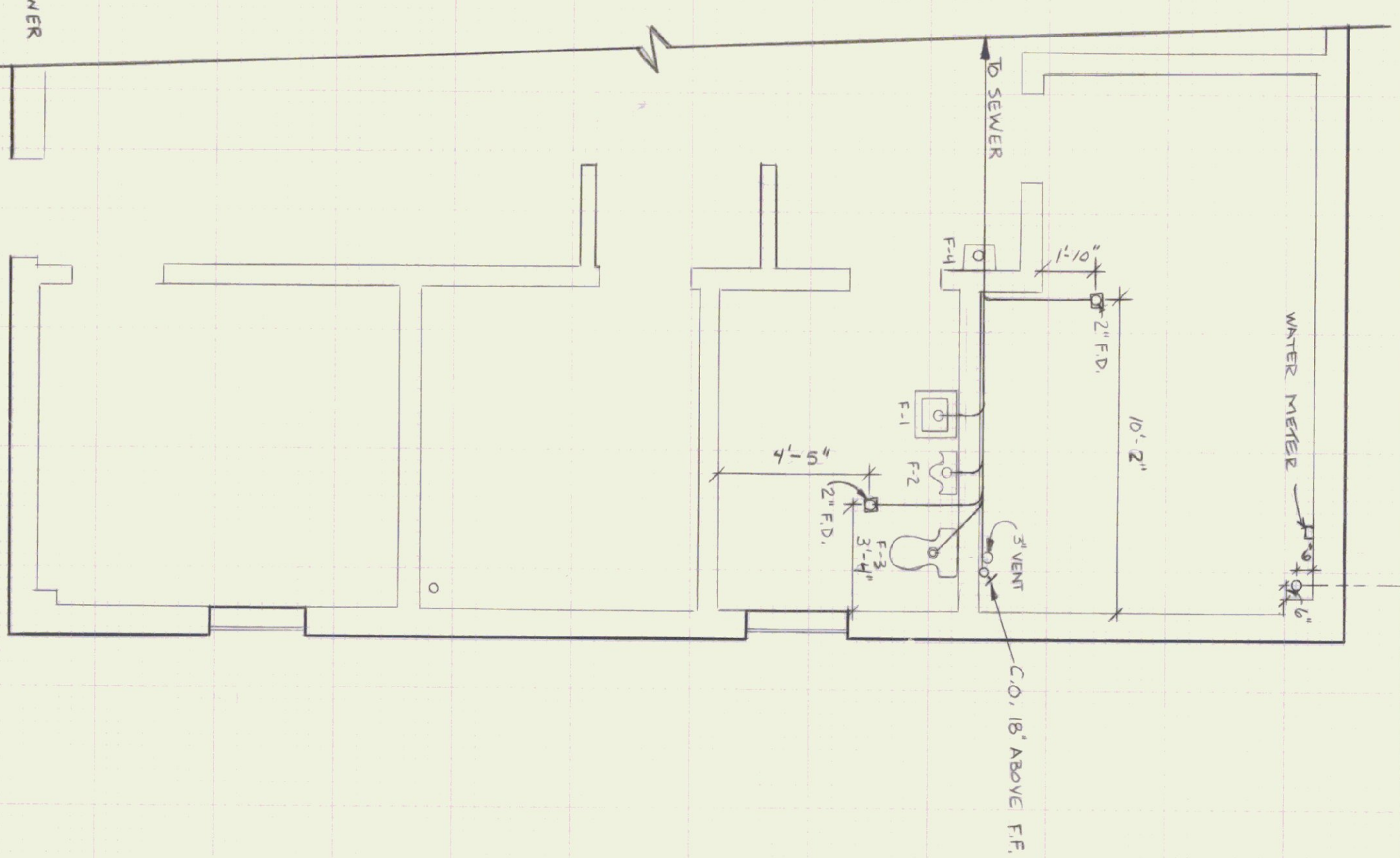
SANITARY WASTE 1/2" VENT PLAN SCALE 1/4" = 1'-0"
