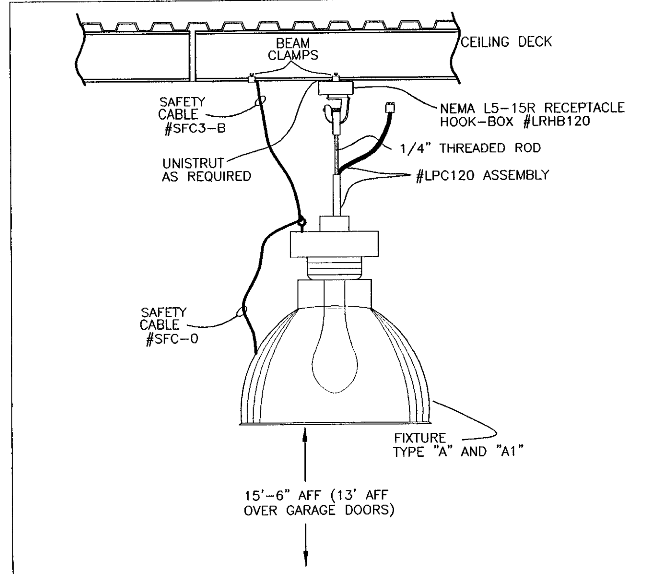
TYPE "A" & "A1" FIXTURE MOUNTING DETAIL NO SCALE
