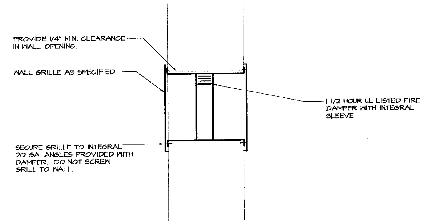
WALL GRILLE WITH FIRE DAMPER NO SCALE
