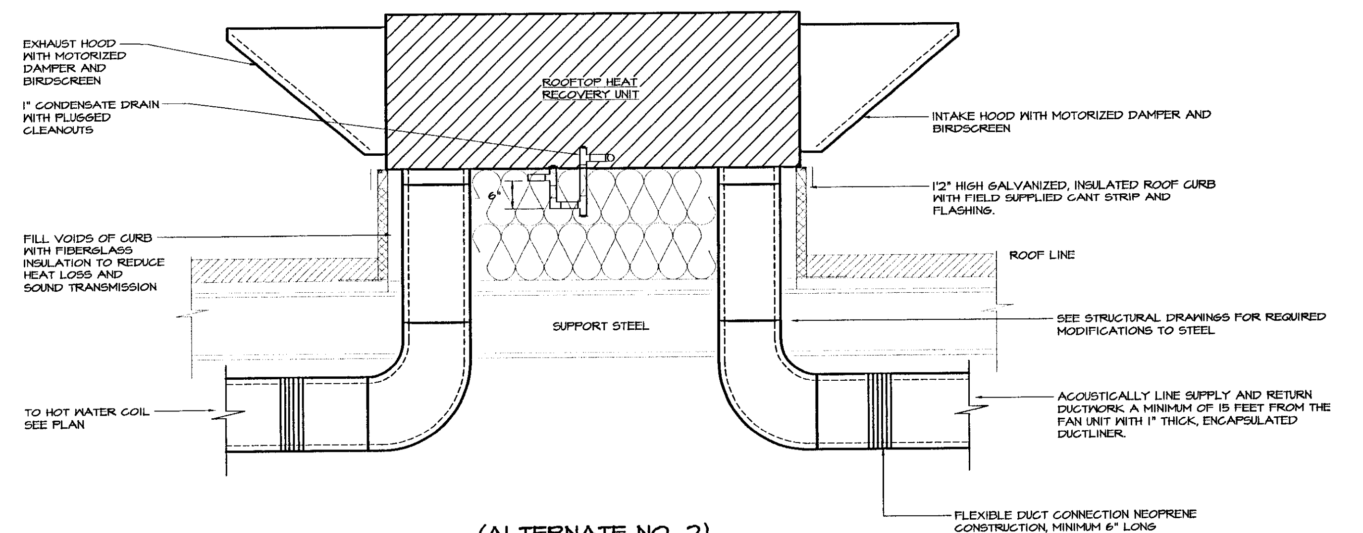
(ALTERNATE NO. 2) ROOFTOP HEAT RECOVERY UNIT DETAIL NOT TO SCALE
