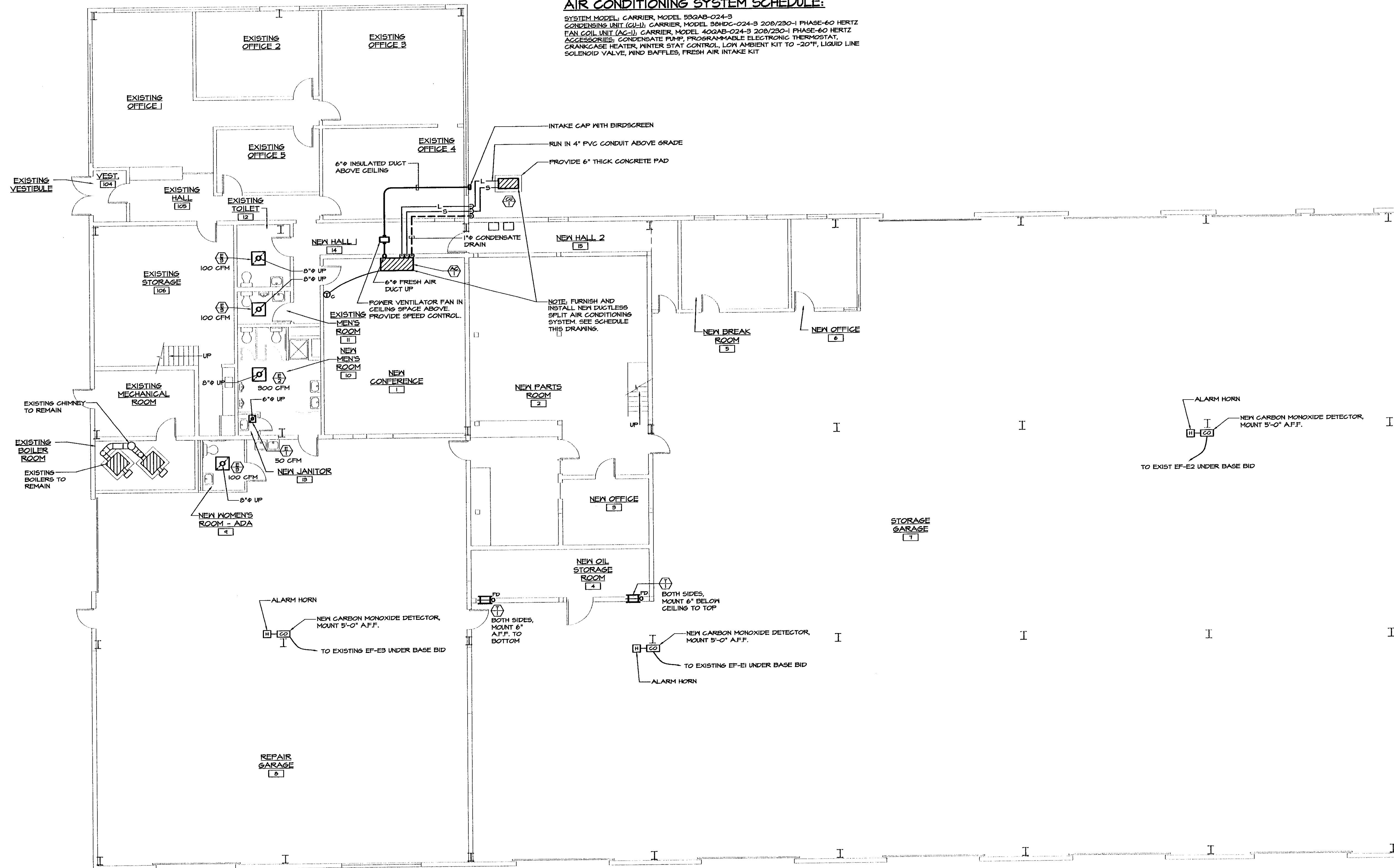
MAIN FLOOR PLAN - NEW VENTILATION BASE BID SCALE: 1/8"=1'-0"
