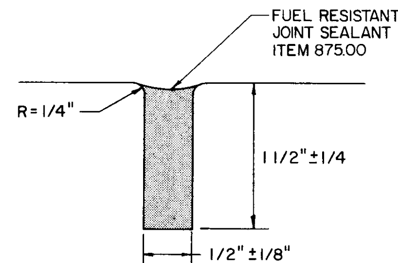
JOINT FILLER DETAIL NO SCALE
