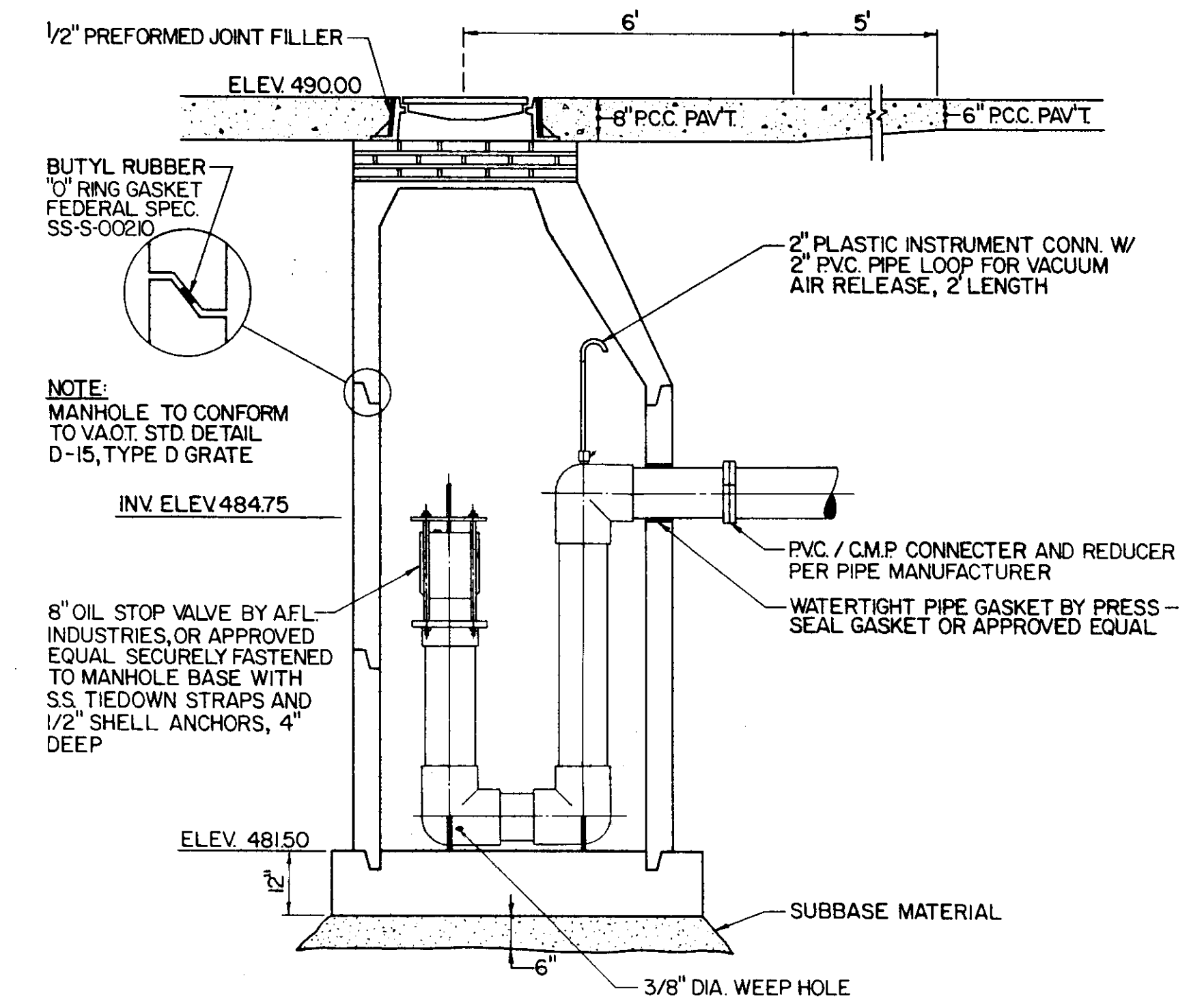
OIL / WATER SEPARATOR NO SCALE
