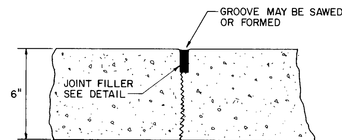
CONTRACTION JOINT DETAIL NO SCALE
