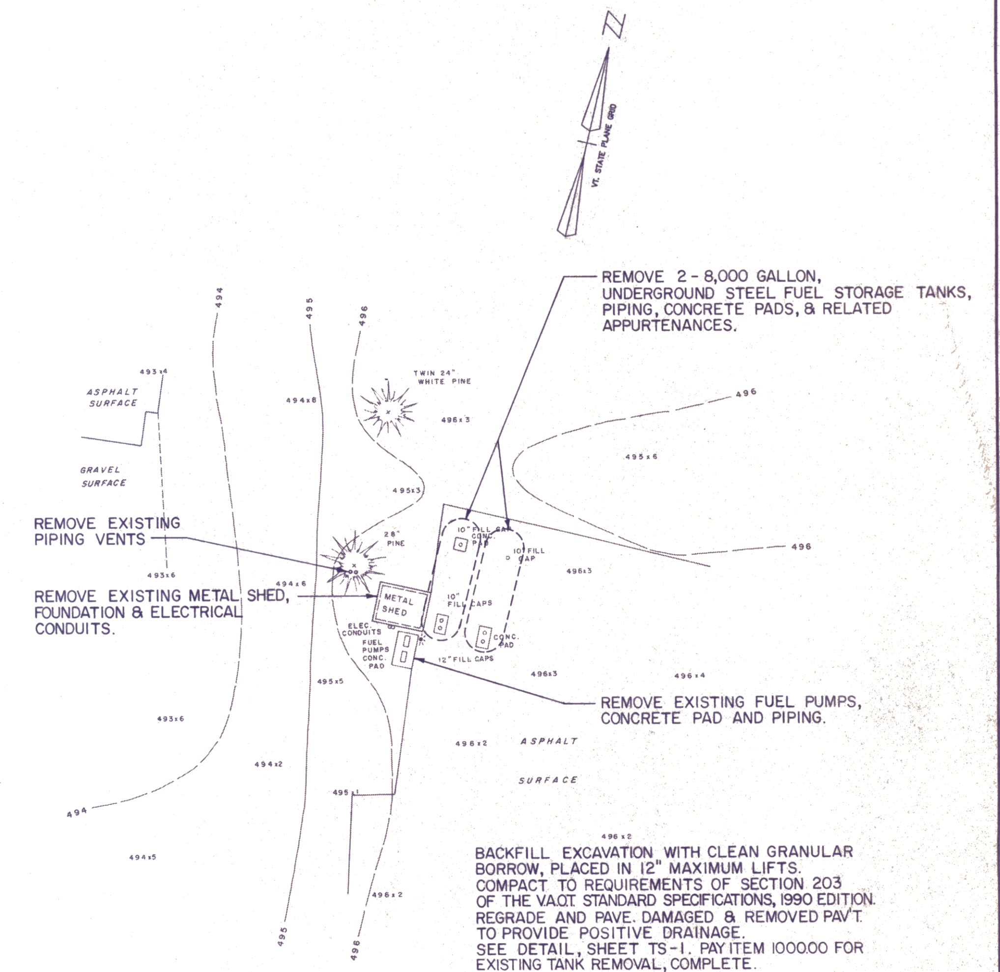
EXISTING STORAGE TANK REMOVAL PLAN SCALE 1" = 20'
