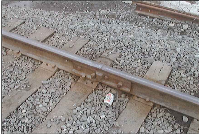
STEP JOINT
