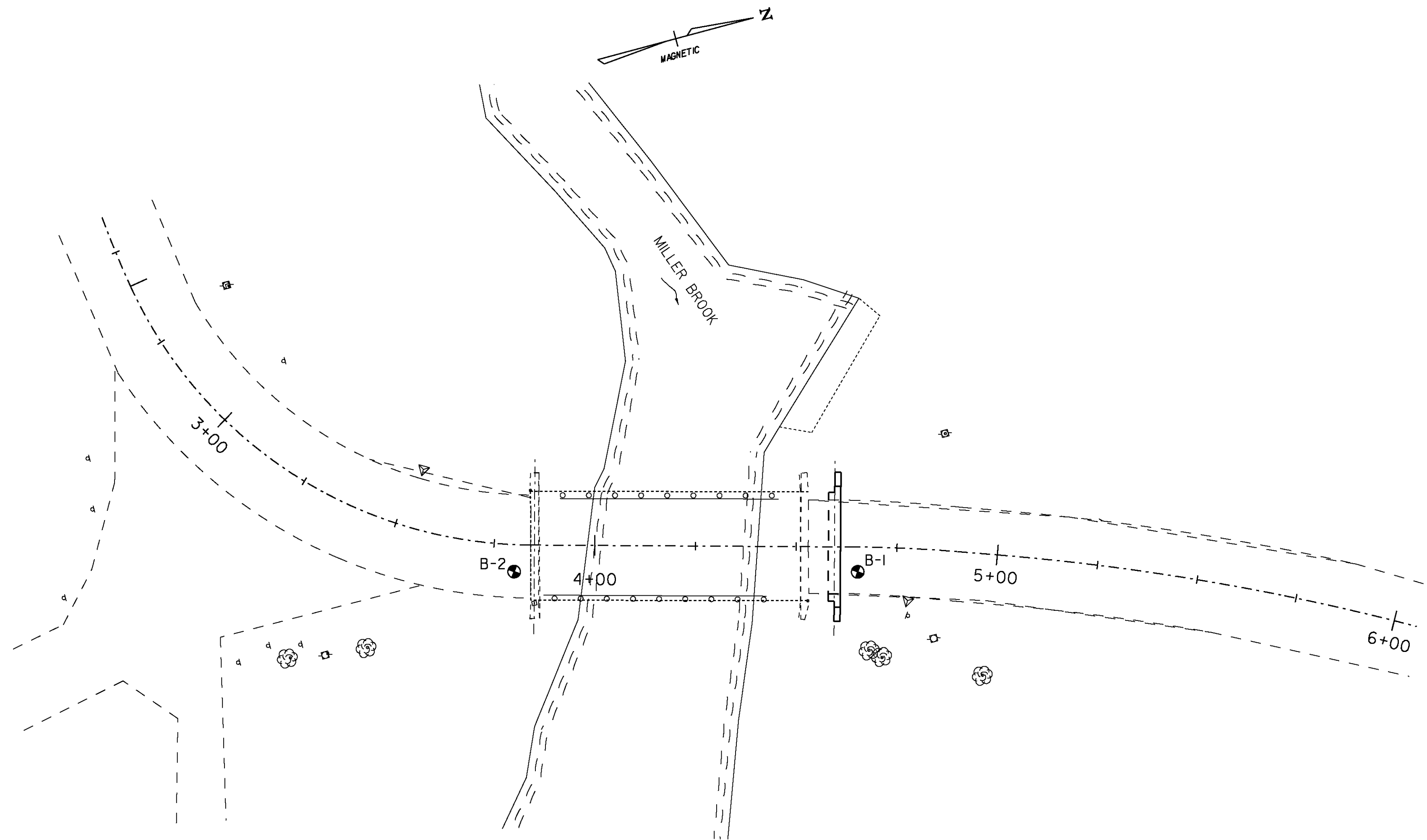
PLAN SCALE 1" = 20'-0" 20 0 20
