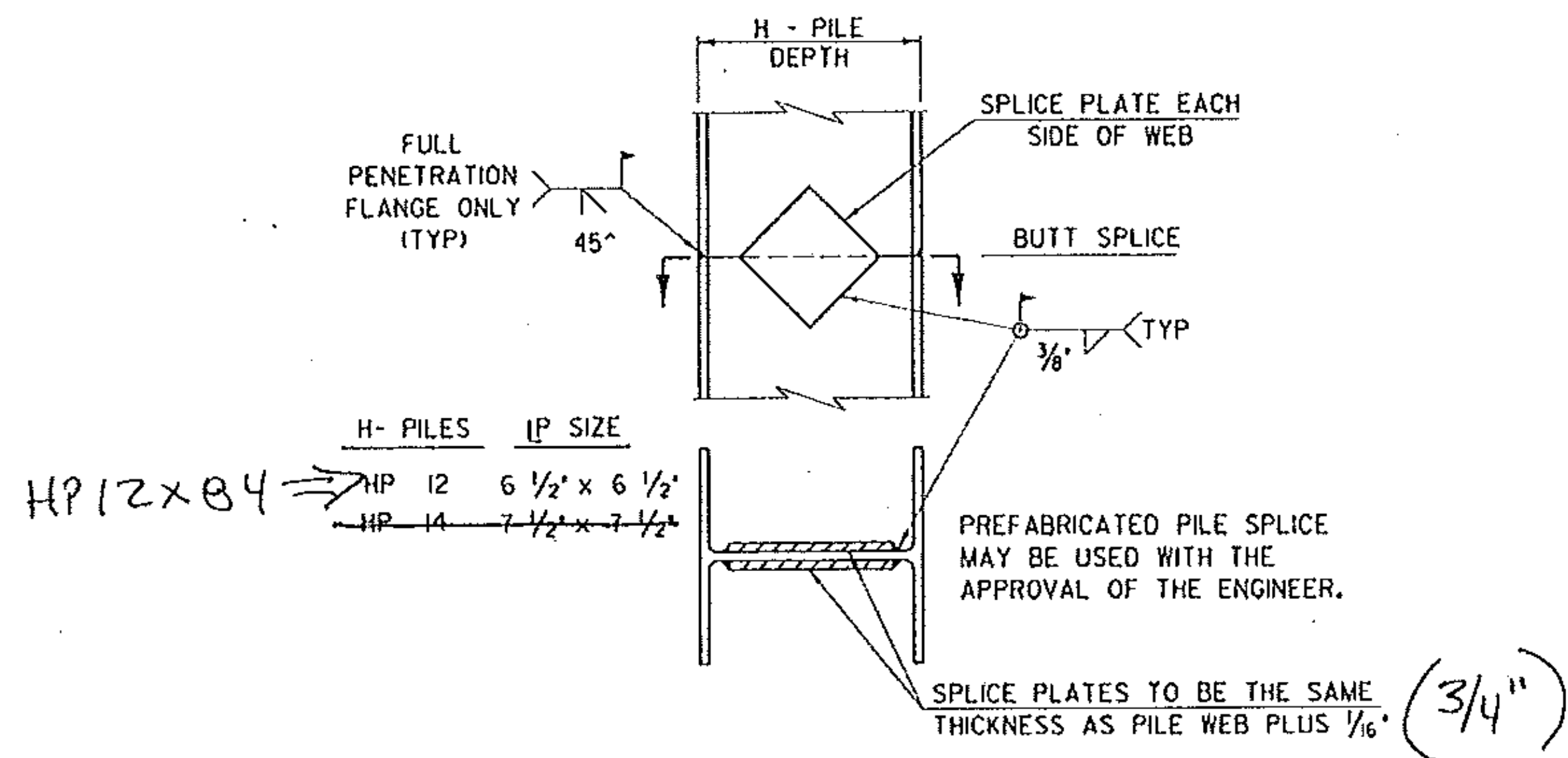
DETAIL OF PILE SPLICE
