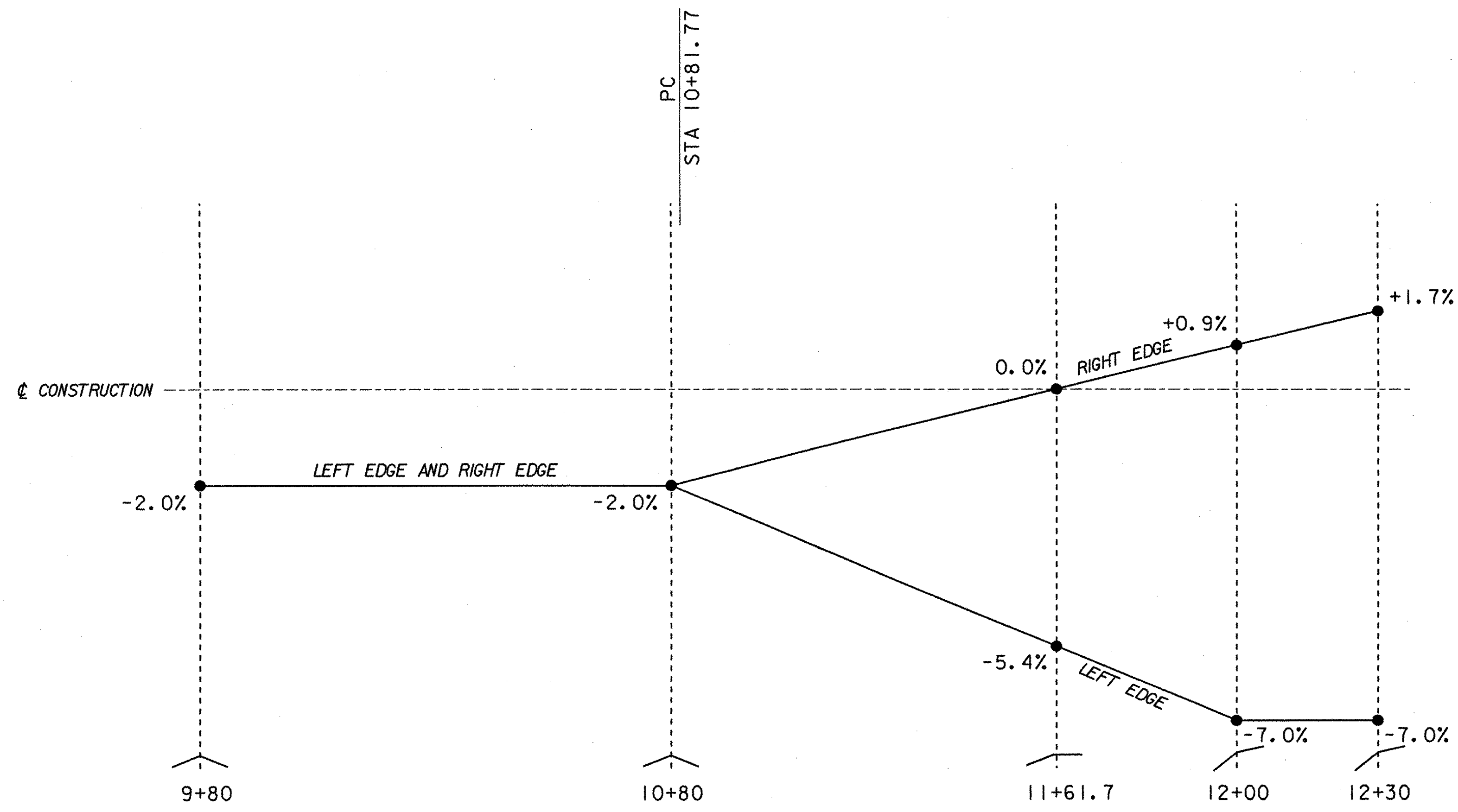
BANKING DIAGRAM
