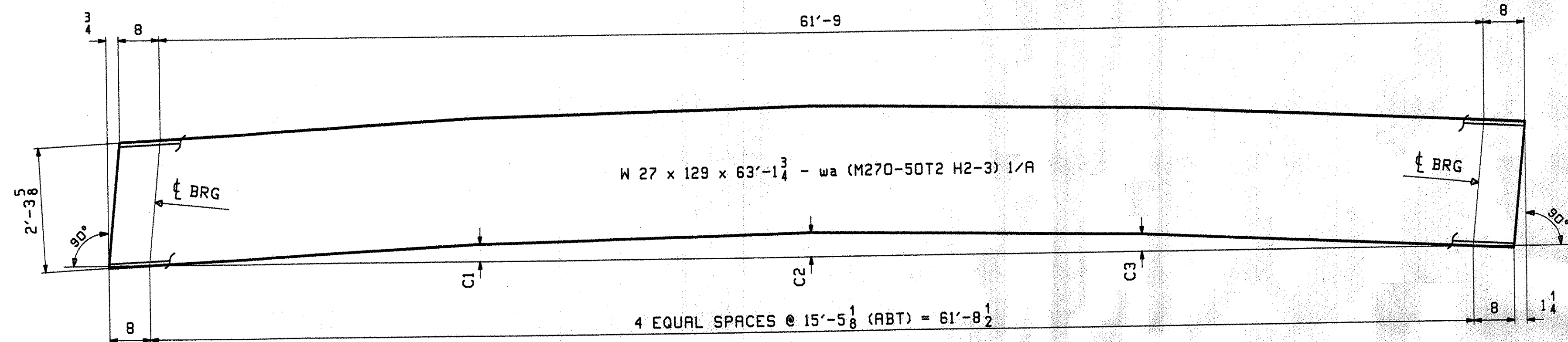
CAMBER DIAGRAM FOR 1S1A THRU 6S6A
