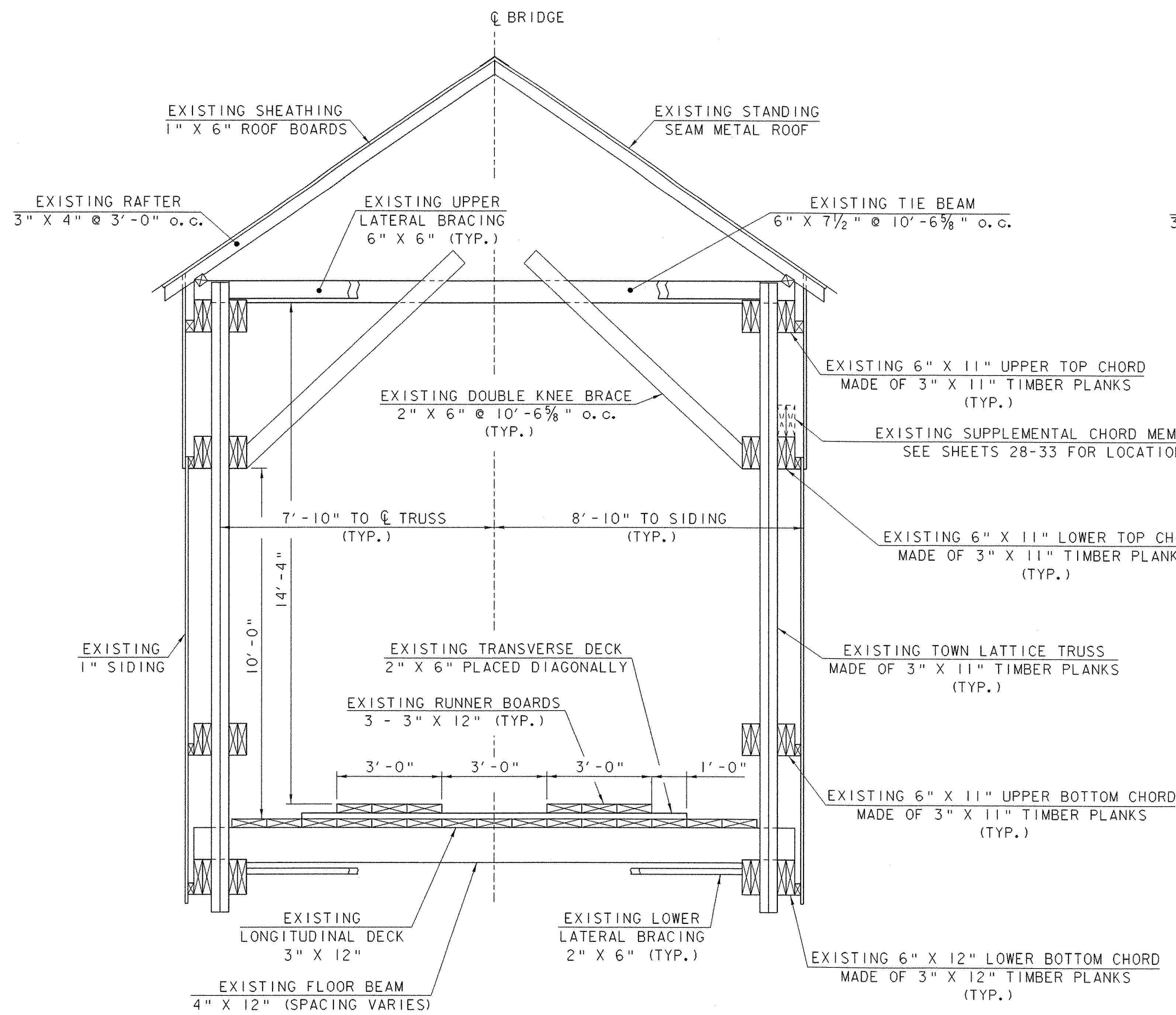
EXISTING BRIDGE TYPICAL SECTION
