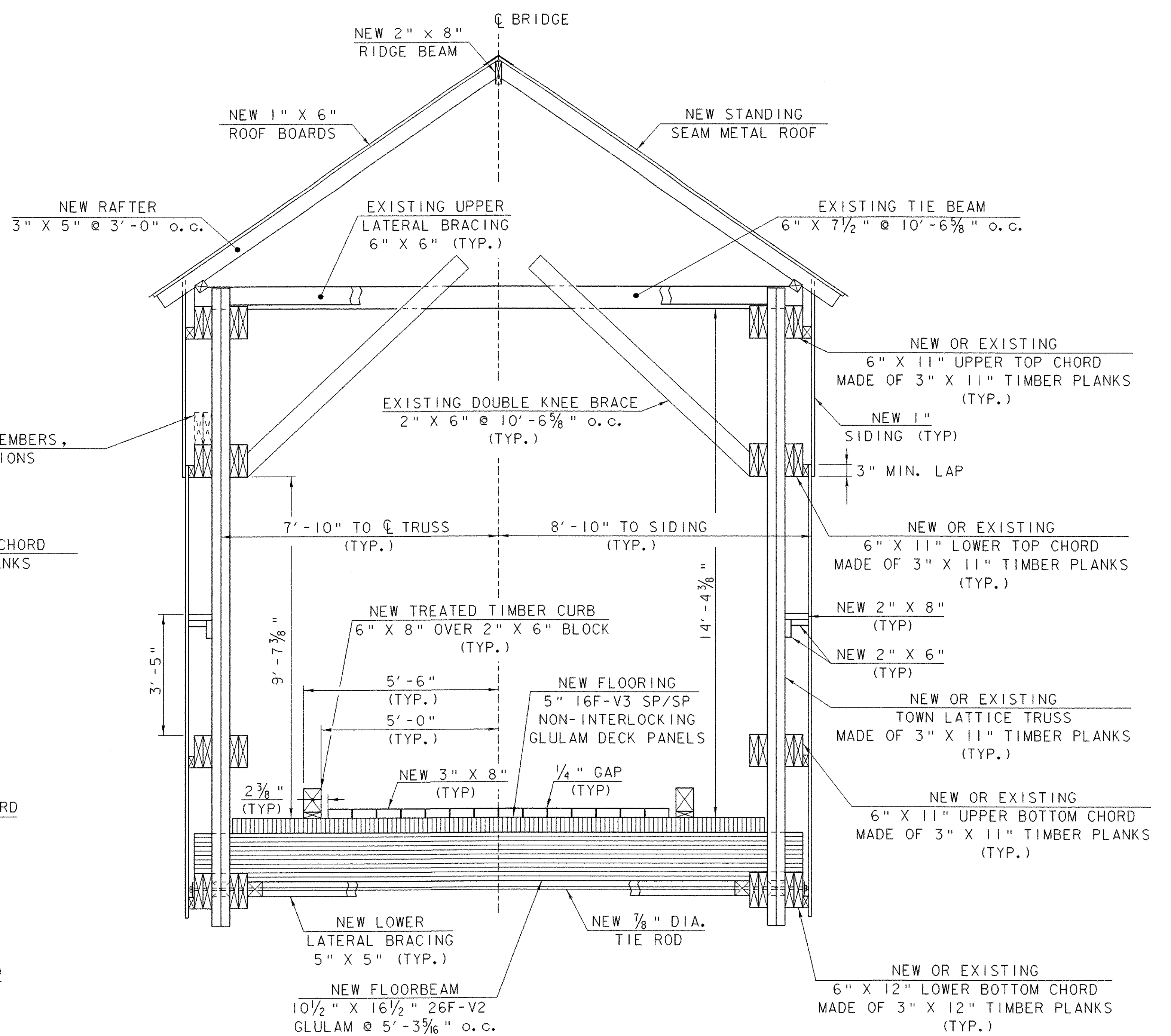
REHABILITATED BRIDGE TYPICAL SECTION
