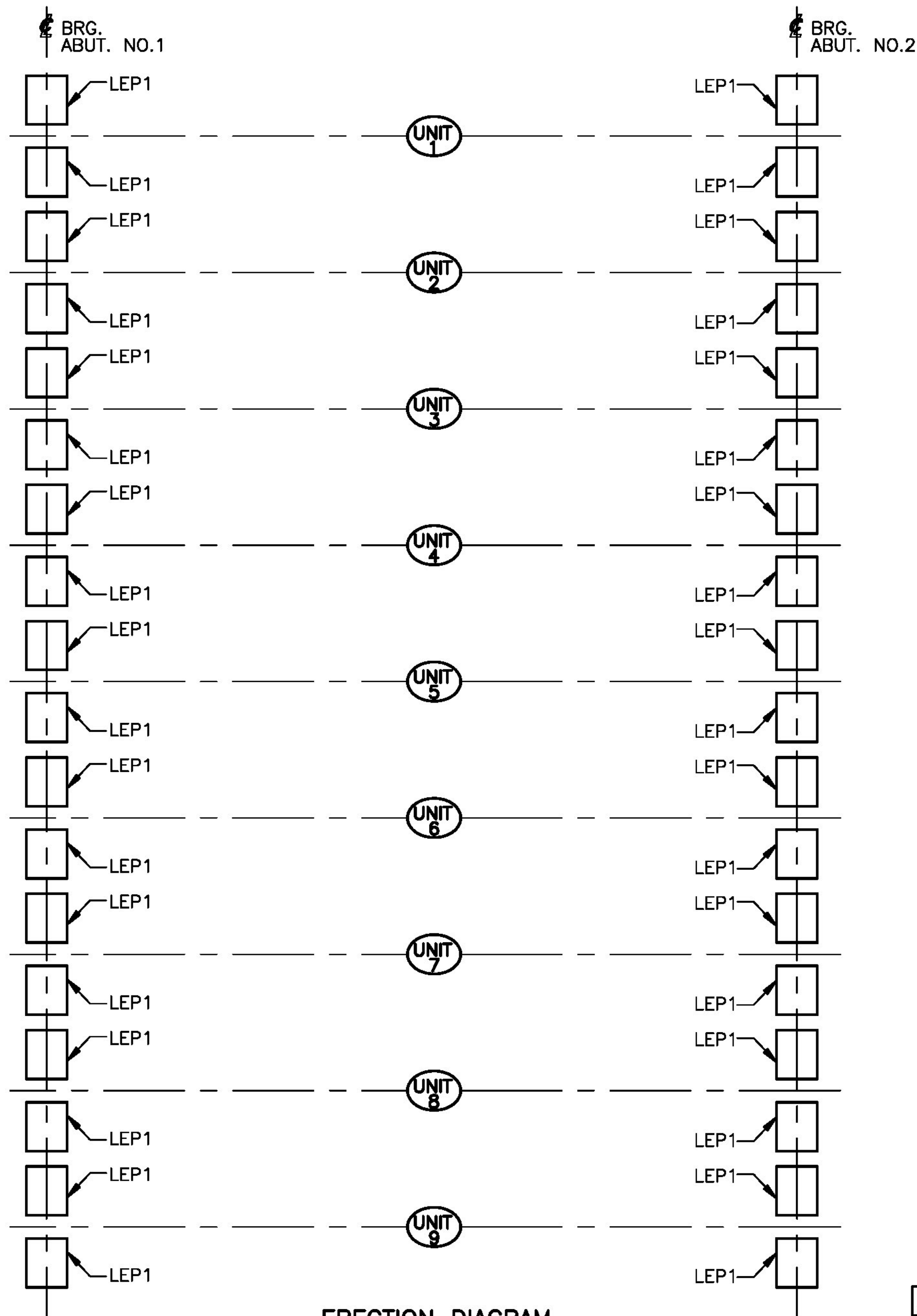
ERECTION DIAGRAM
