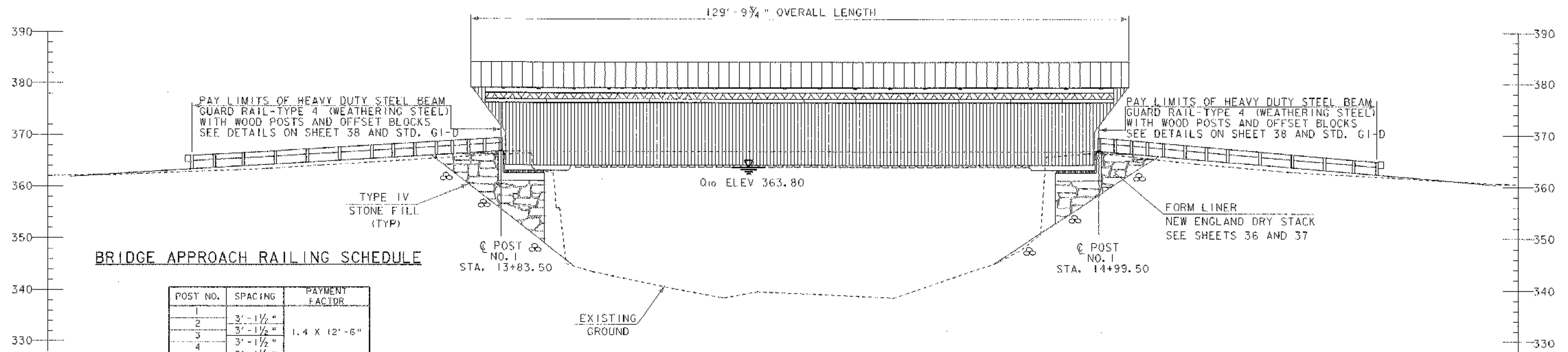
UPSTREAM ELEVATION SCALE 1" = 10'-0"
