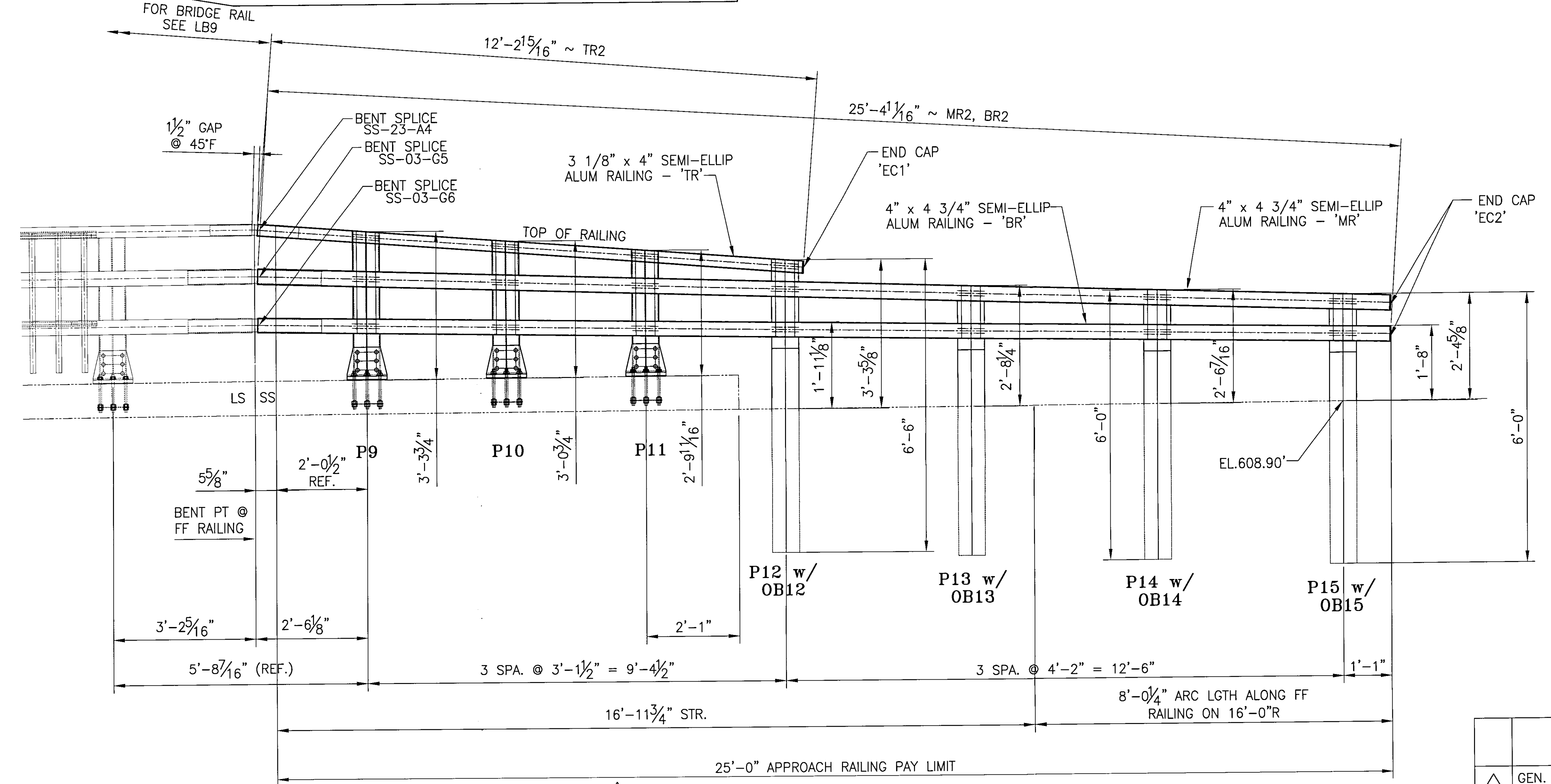
1 INSIDE ELEVATION OF SW APPROACH RAIL
