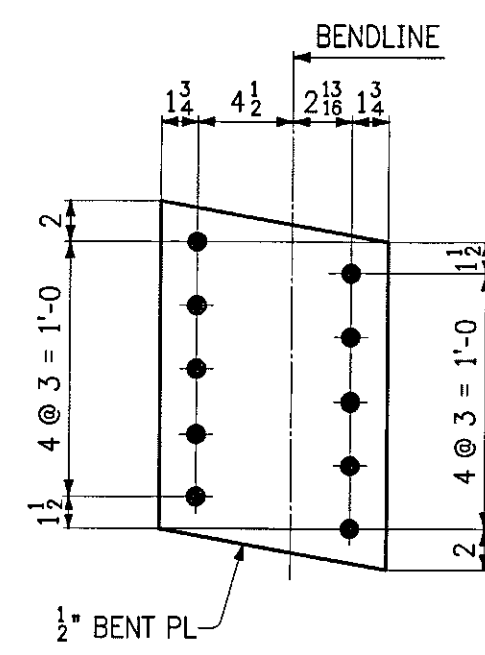
DEVELOPED DETAIL OF BENT PL
