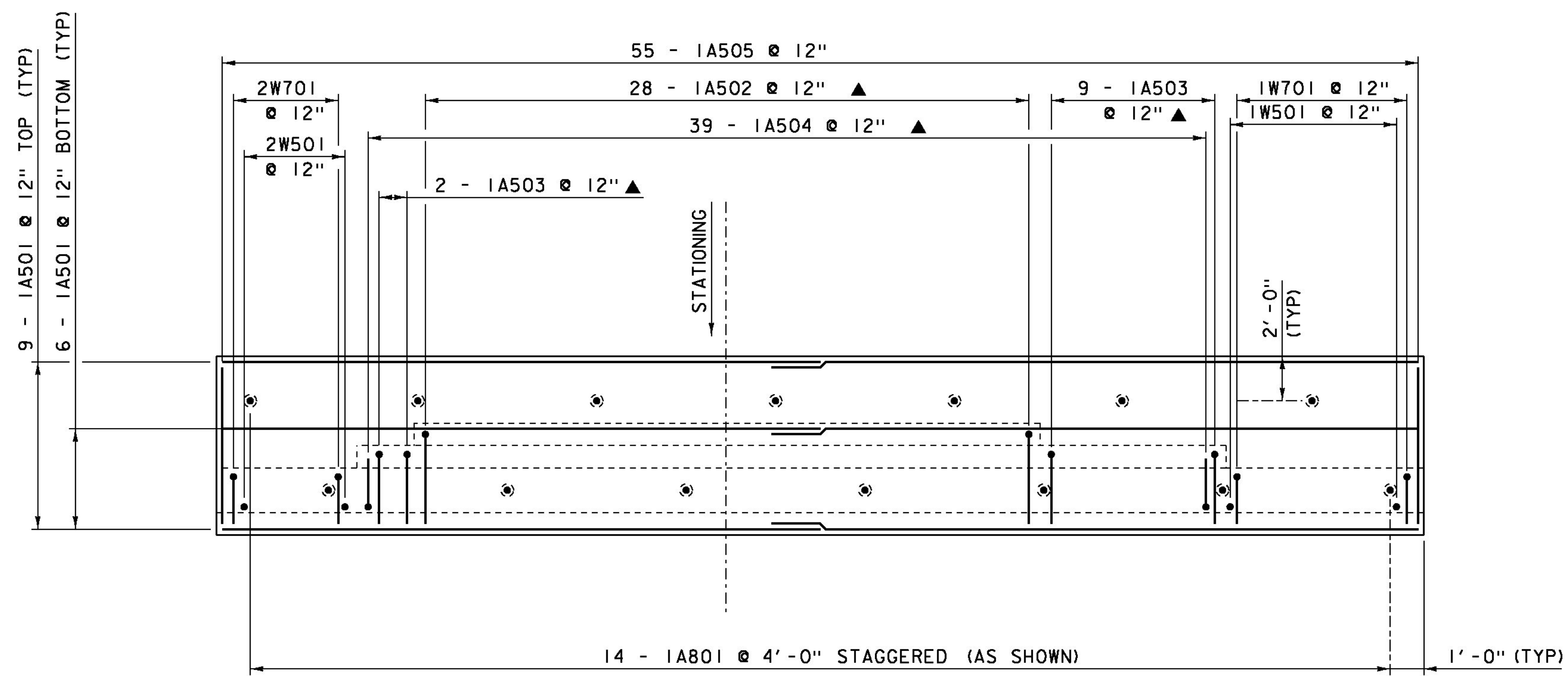
ABUTMENT #1 FOOTING REINFORCING PLAN
