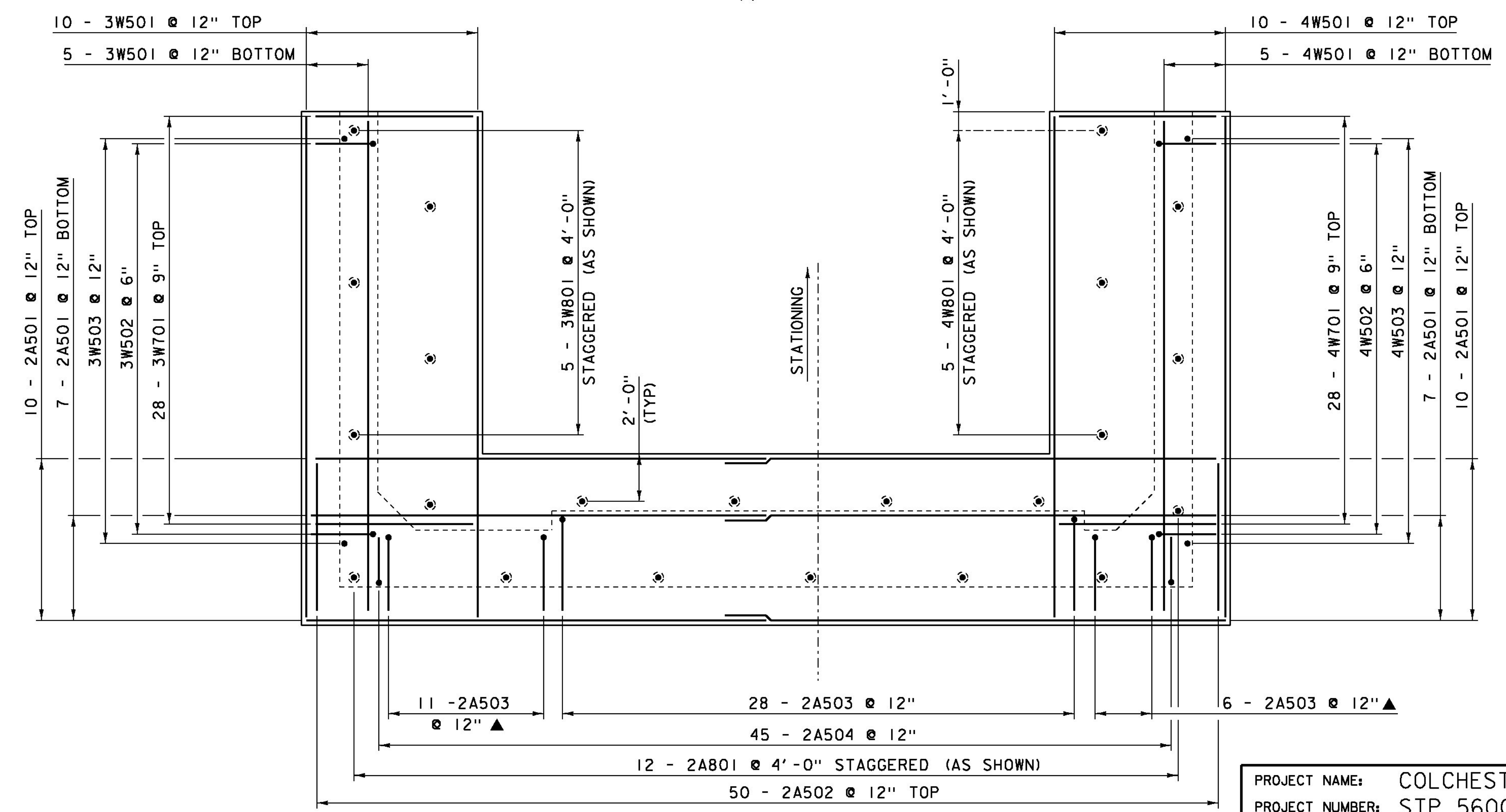
ABUTMENT #2 FOOTING REINFORCING PLAN
