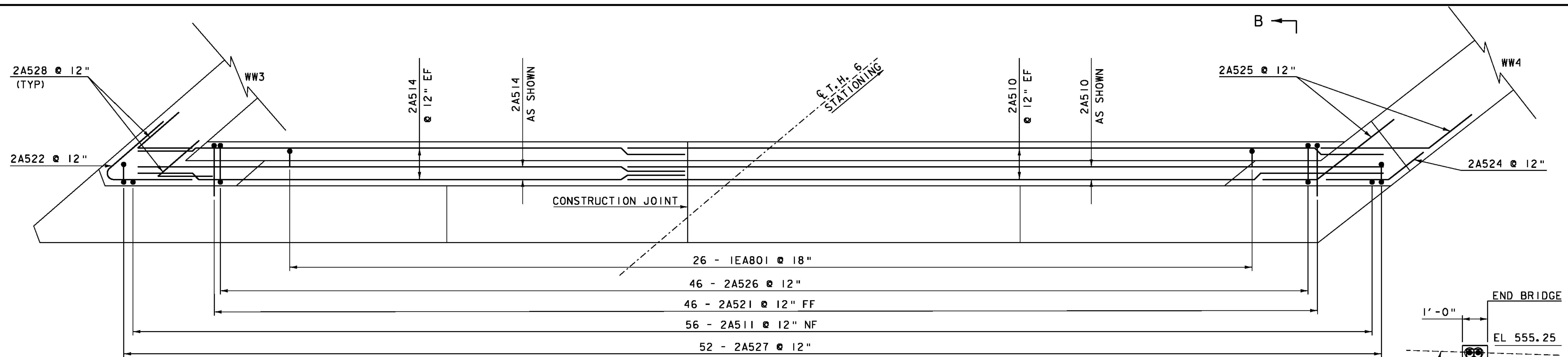
ABUTMENT 2 BACKWALL PLAN VIEW SCALE 1/2" = 1'-0"
