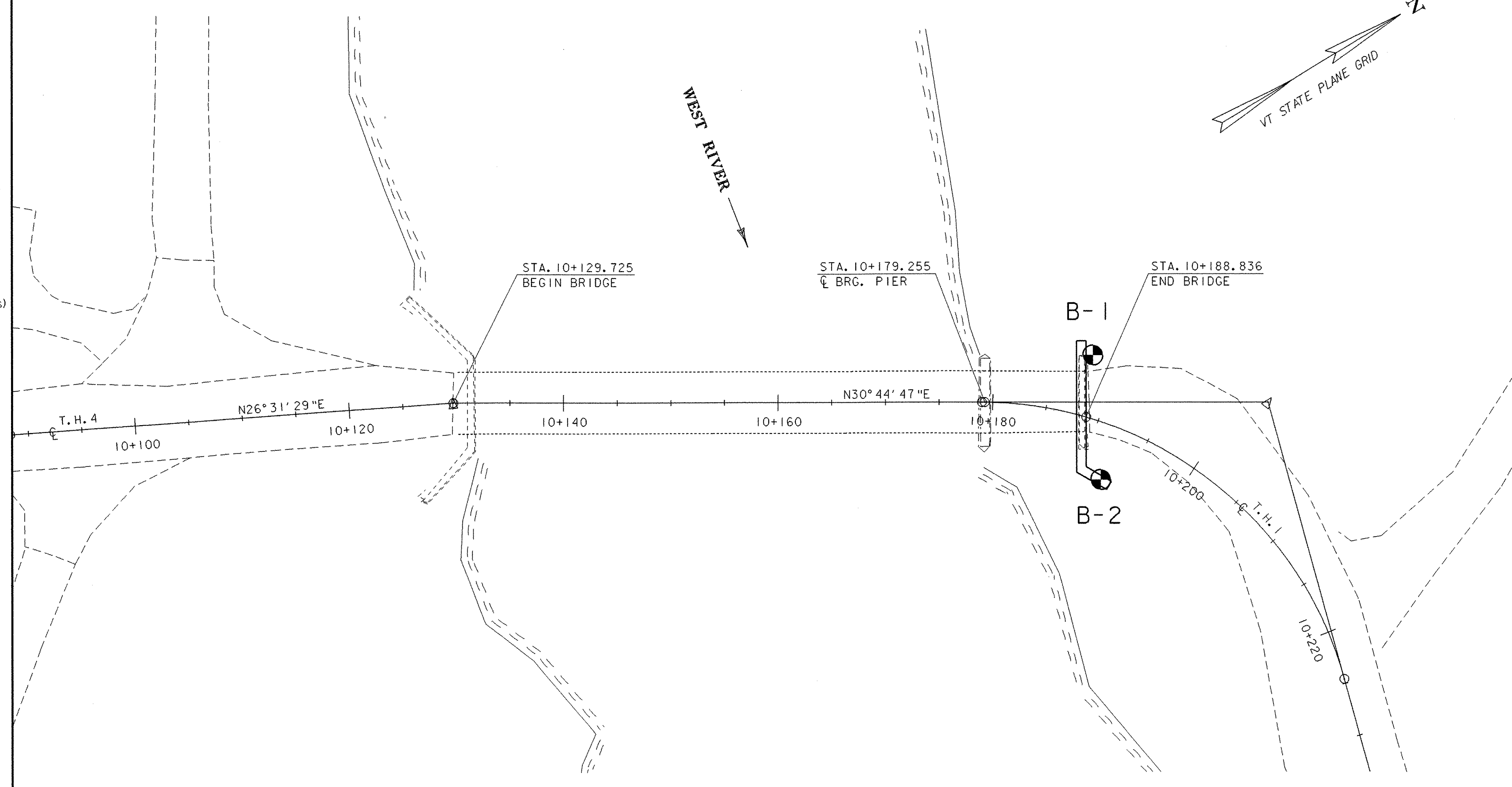
BORING PLAN SCALE = 1:250
