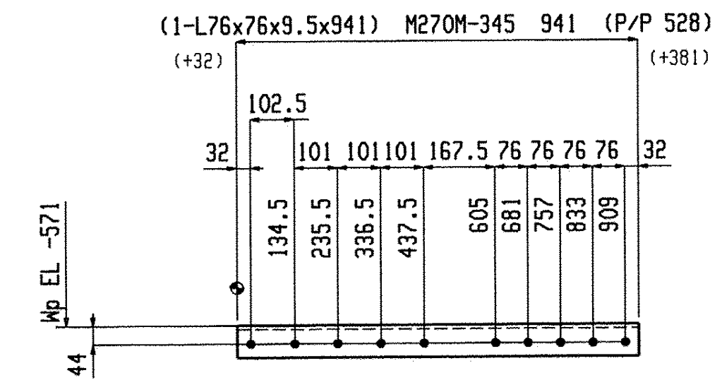
14 HORIZONTAL BRACES HB6
