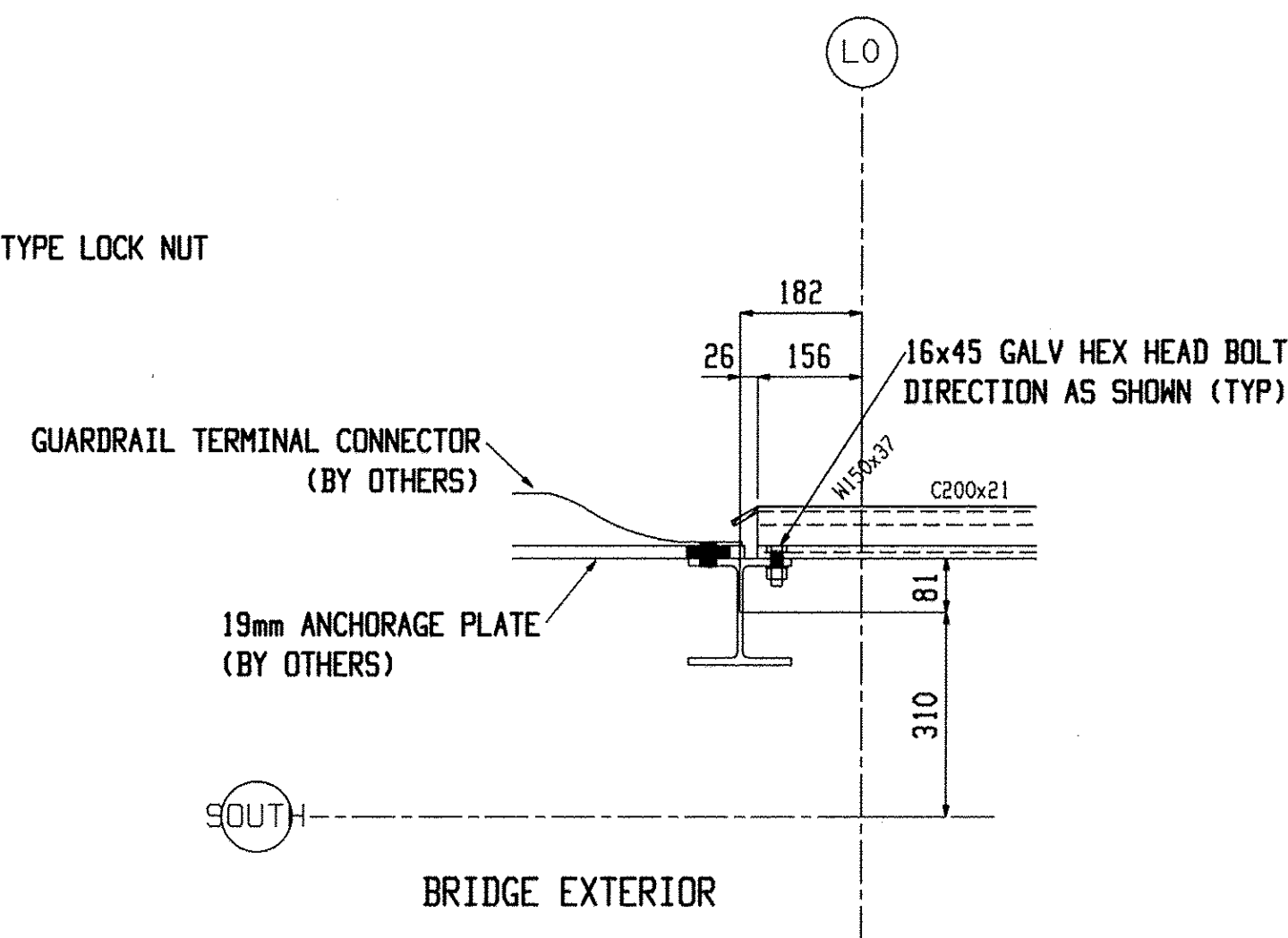
SECTION 8 Elevation: 775 (U.N.)
