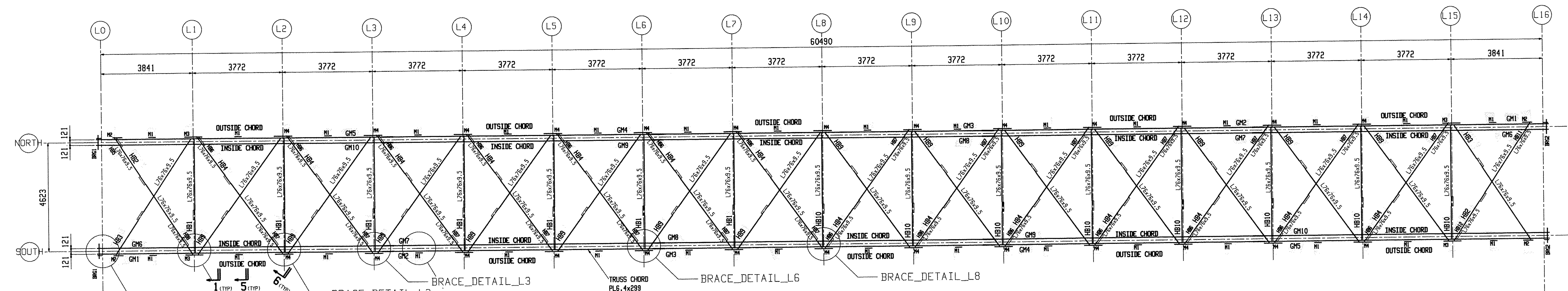
DECK BRACING Elevation: -571 (U.N.) TRUSS IS SYMMETRICAL ABOUT L8 LINE
