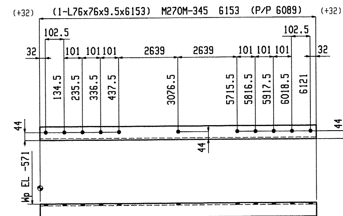
14 HORIZONTAL BRACES HB9
