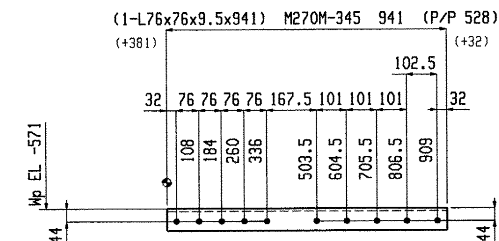
14 HORIZONTAL BRACES HB7
