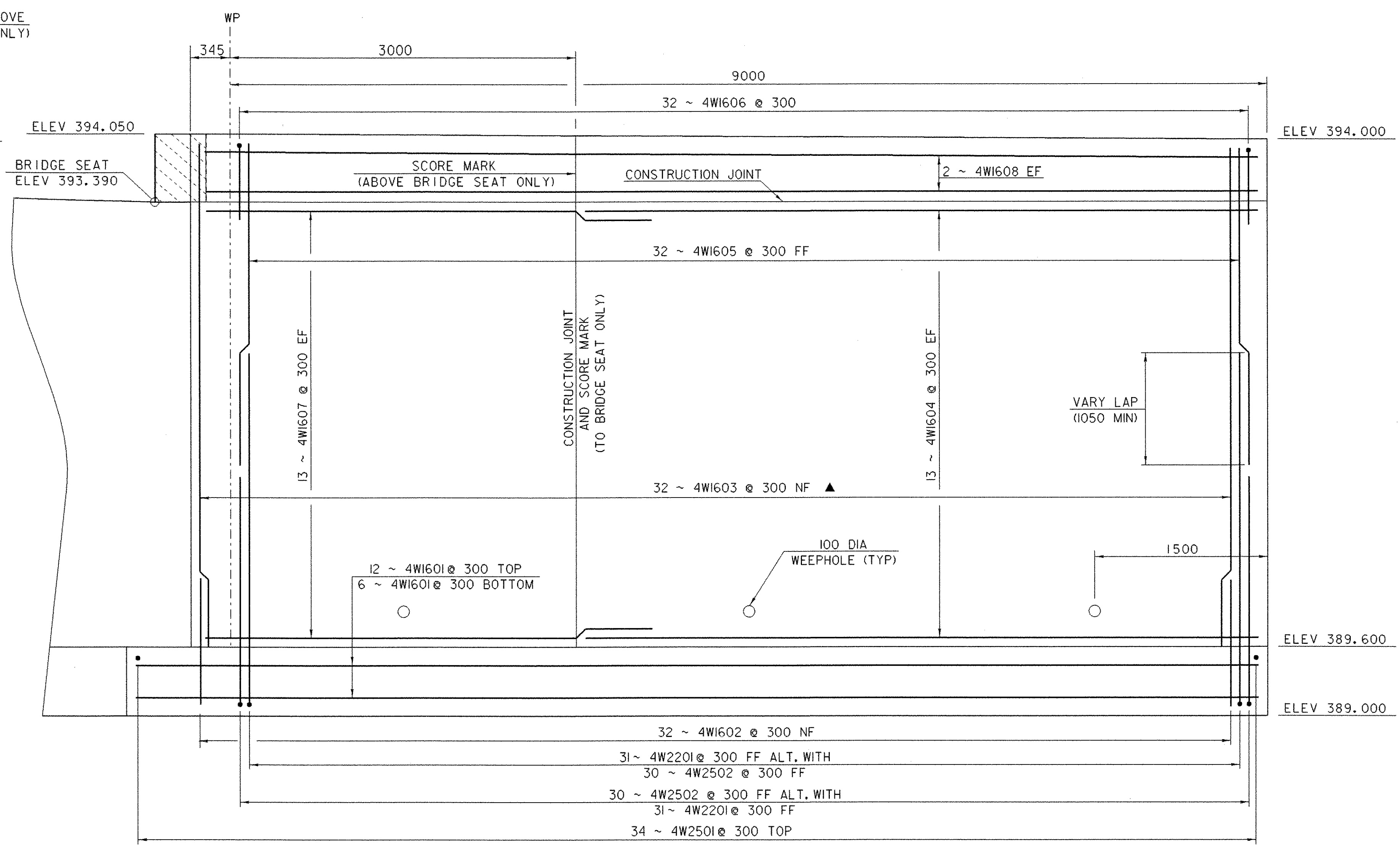
WINGWALL #4 ELEVATION SCALE: 1:25
