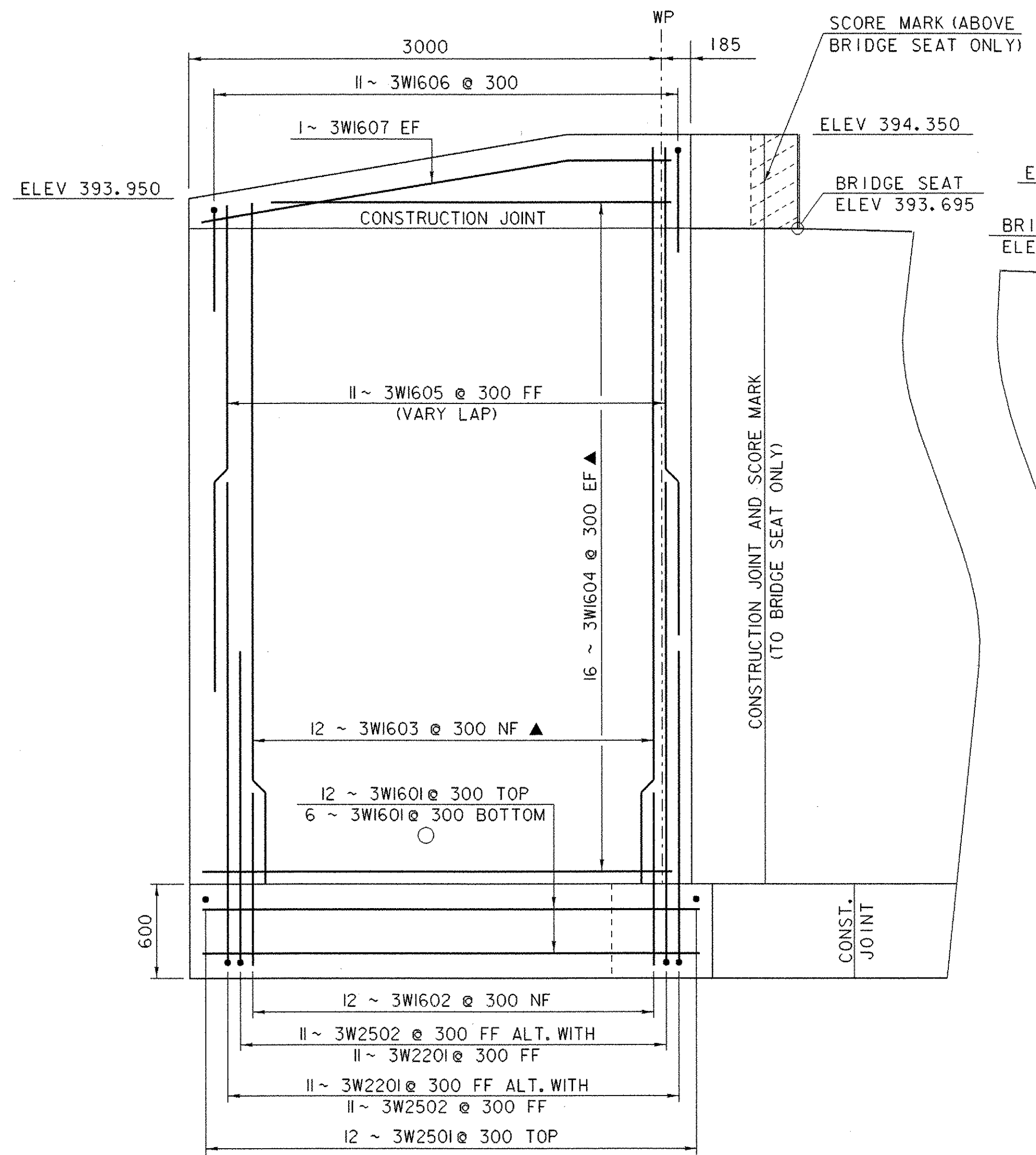
WINGWALL #3 ELEVATION SCALE: 1:25
