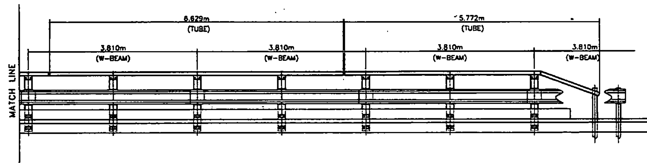
NORTH ELEVATION LOOKING AT RAIL FROM C OF ROAD
