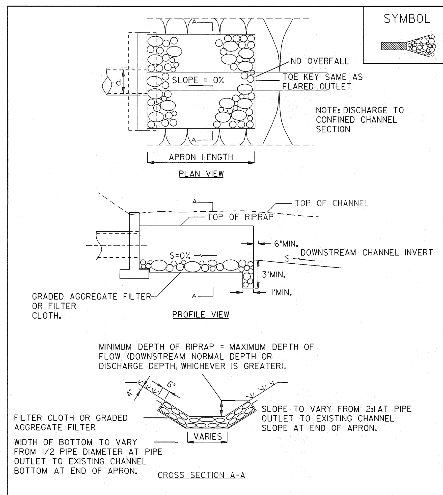
RIPRAP OUTLET PROTECTION EXAMPLE
