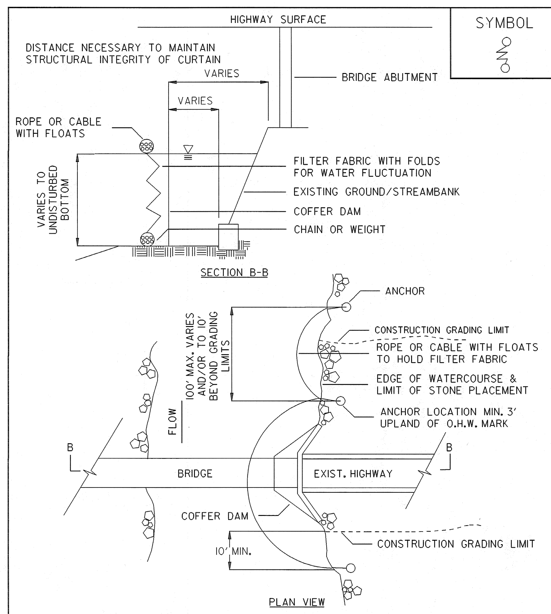
TURBIDITY CURTAIN
