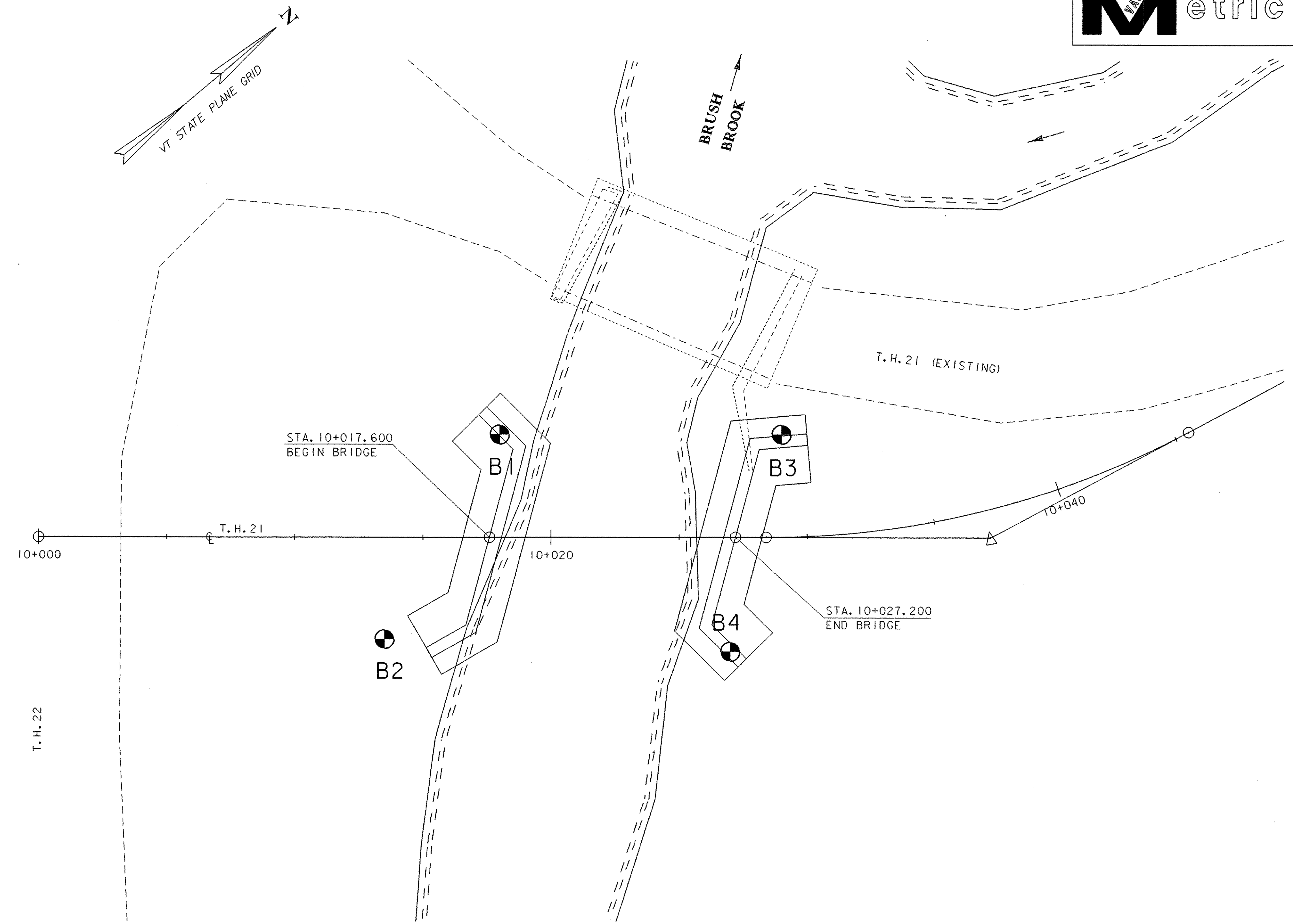
BORING PLAN
