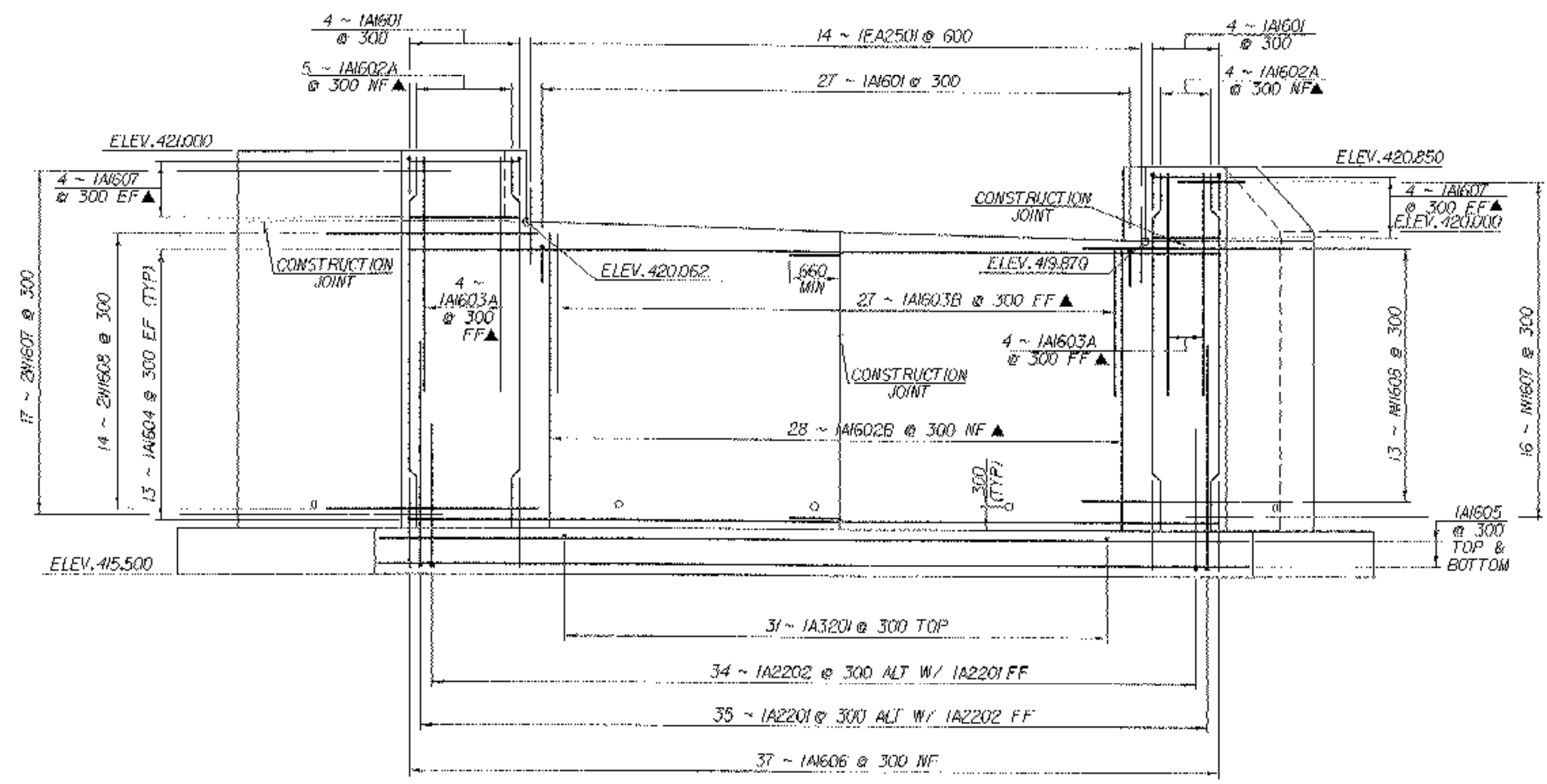
ABUTMENT NO. 1 ELEVATION
