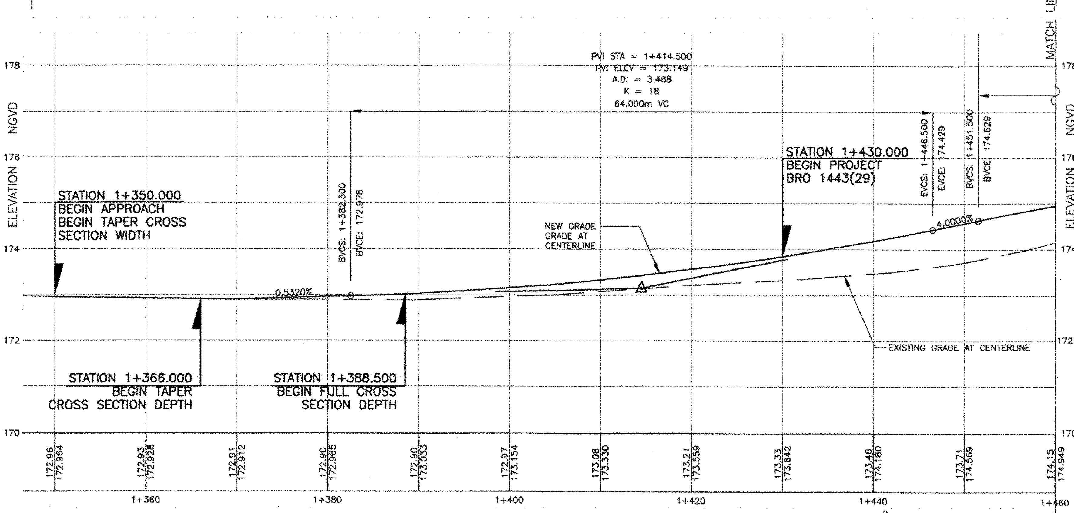
PROFILE SHEET SCALE HORIZ. 1:250 VERT. 1:50
