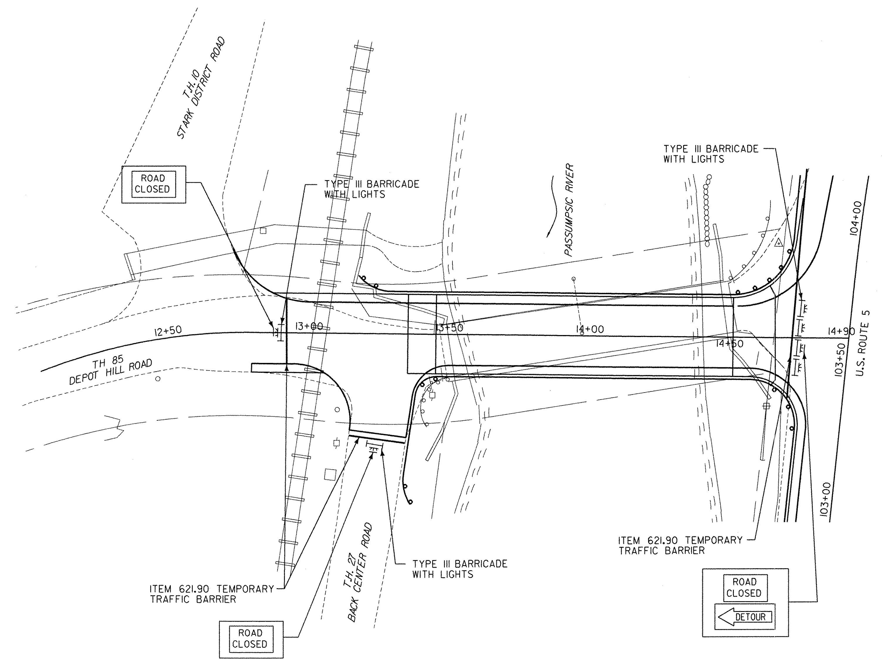
DETAIL A
