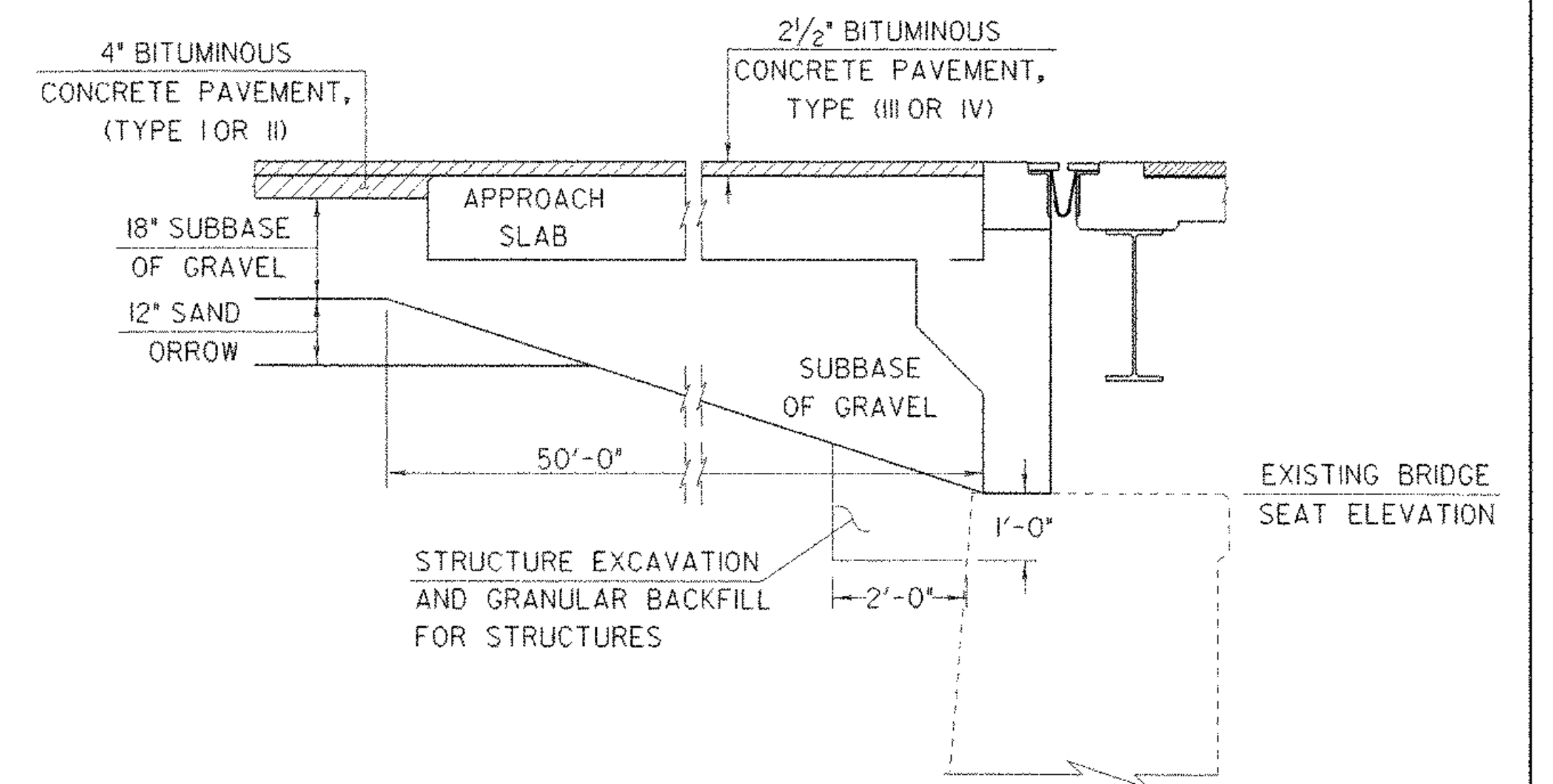
ABUTMENT MATERIAL TRANSITION (TYPICAL OF BOTH ABUTMENTS)
